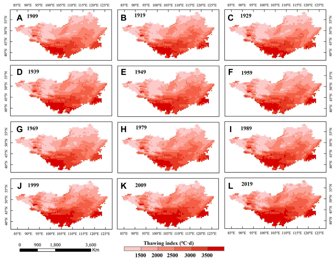
FIGURE 6 | Decadal spatial changes in the air thawing index on the Mongolian Plateau from 1901 to 2019. Labels like (A–L) represent the spatial variation of the air thawing index for each decade from 1901 to 2019.
