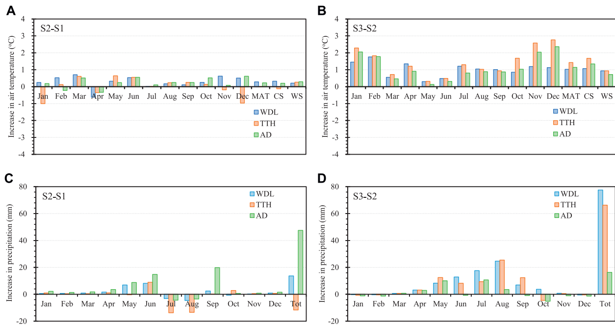
FIGURE 5 | Periodic changes in mean monthly, mean annual (MAT), cold season (CS), and warm season (WS) air temperature at the three weather stations. (A) Temperature changes from stage 1 (S1, before 1979) to stage 2 (S2, 1980–1999) and (B) from stage 2 (S2, 1980–1999) to stage 3 (S3, 2000–2019). Periodic changes in mean monthly and total precipitation (Tot) at the three weather stations. (C) Precipitation changes from stage 1 (S1, before 1979) to stage 2 (S2, 1980–1999) and (D) from stage 2 (S2, 1980–1999) to stage 3 (S3, 2000–2019).
