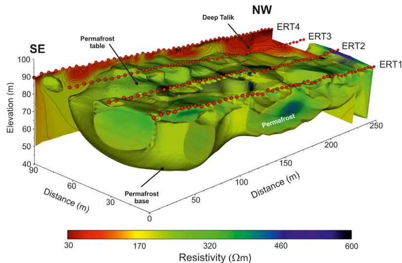
FIGURE 10 | Permafrost volume obtained by a 3D interpolation of the resistivity values higher than 200 \Omega\text{m} over the four ERT sections of Site 1A. Permafrost thickness substantially reduces and becomes discontinuous upon approaching the riverbank.
