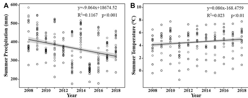
FIGURE 1 | Summer precipitation (A) and air temperature (B) between 2008 and 2018 in all the sites we surveyed in the permafrost region of the Tibetan Plateau. Solid circle, alpine meadow; blank circle, alpine steppe.
