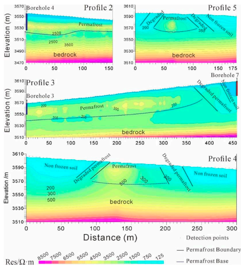
FIGURE 9 OCTEM sounding profiles in Mahan Mountain.
