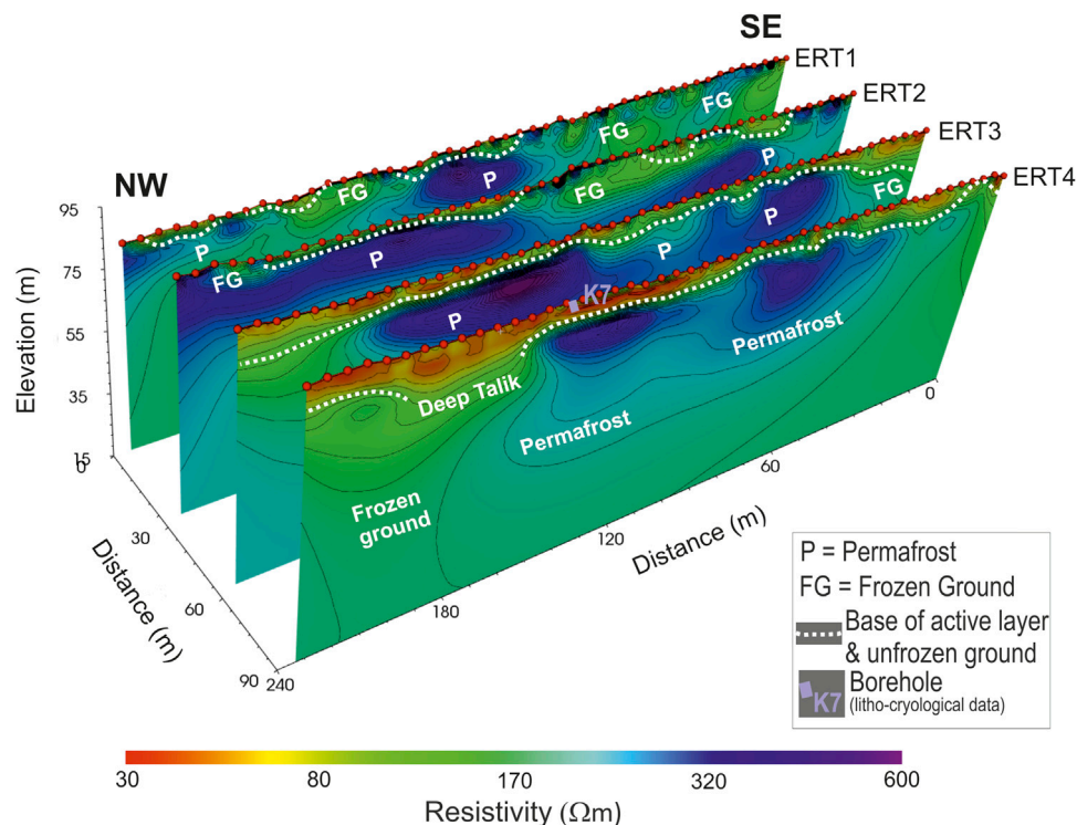
FIGURE 8 | 3D representation of the ERT sections in Site 1A. According to the CRIM analysis and to the resistivity-cryological patterns, the interpretation of the active layer and unfrozen ground bottom (white dashed line) is marked by a resistivity value of 100 \Omega\text{m} . This interpretation, together with the topographic surface (highlighted by red dots representing electrodes deployed during the acquisition), was used to build the ALT and UGT map shown in Figure 9 . The talik, permafrost, and frozen and unfrozen ground areas are also highlighted.
