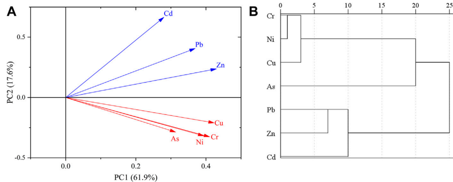
FIGURE 1 | Principal component analysis (A) and cluster analysis (B) for sources of HMs. Loadings larger than 0.50 are displayed in the principal component analysis.
