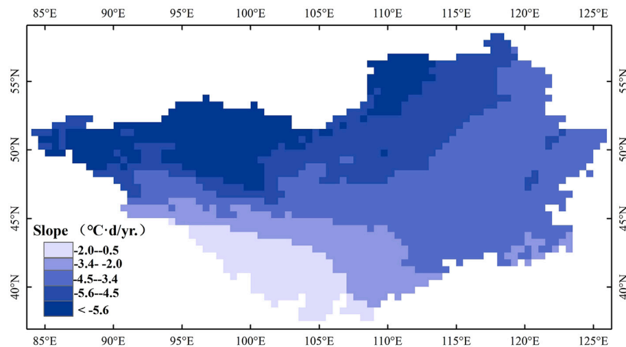
FIGURE 7 | Sen's slope of the freezing index over the Mongolian Plateau from 1901 to 2019.
