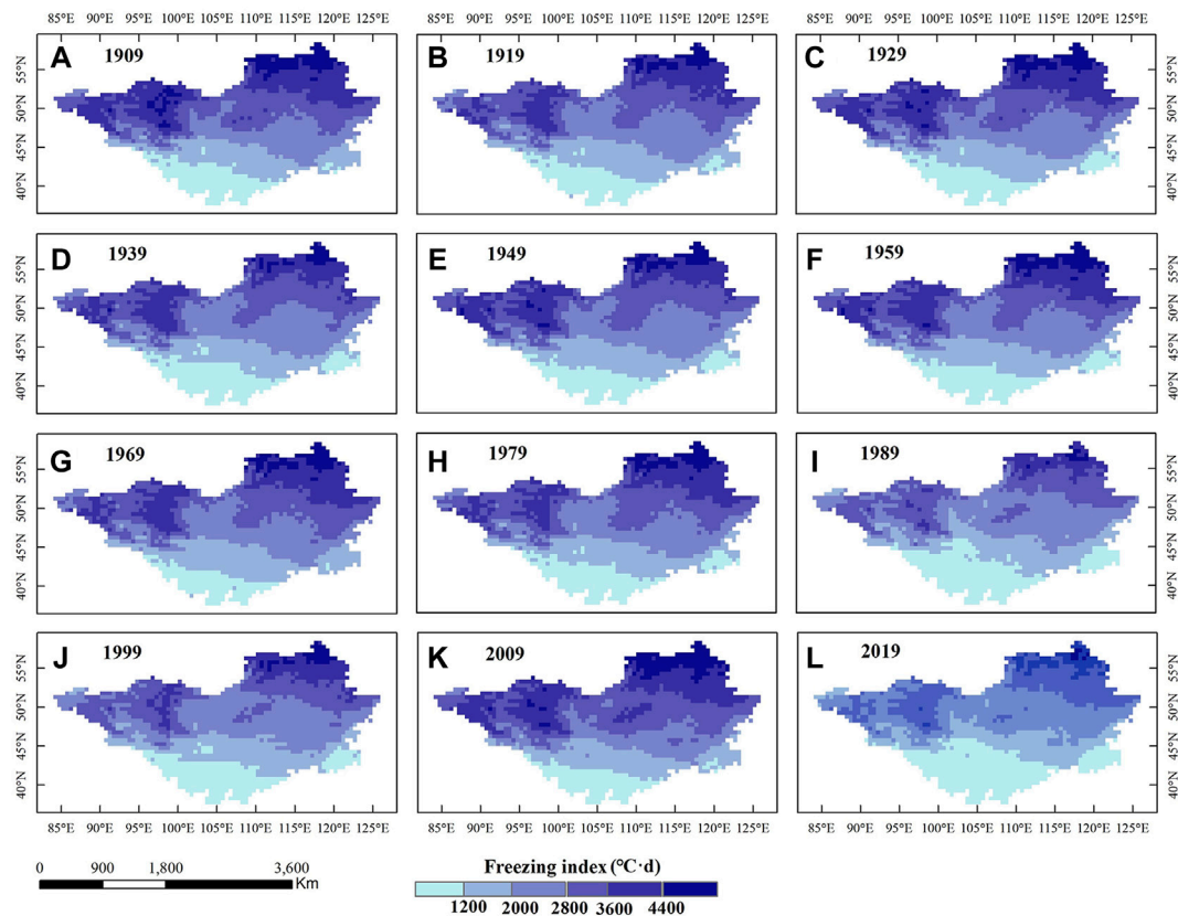
FIGURE 4 | Decadal spatial changes in the air freezing index on the Mongolian Plateau from 1901 to 2019. Labels like (A–L) represent the spatial variation of the air freezing index for each decade from 1901 to 2019.
