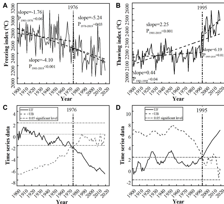
FIGURE 5 | Interannual variation in the freezing (A) and thawing (B) index and the change point of the freezing (C) and thawing (D) index from 1901 to 2019 on the Mongolian Plateau.
