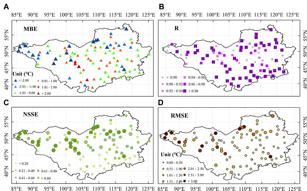
FIGURE 3 | Spatial distribution of four error indicators, including MBE (A), R (B), NSSE (C), and RMSE (D).
