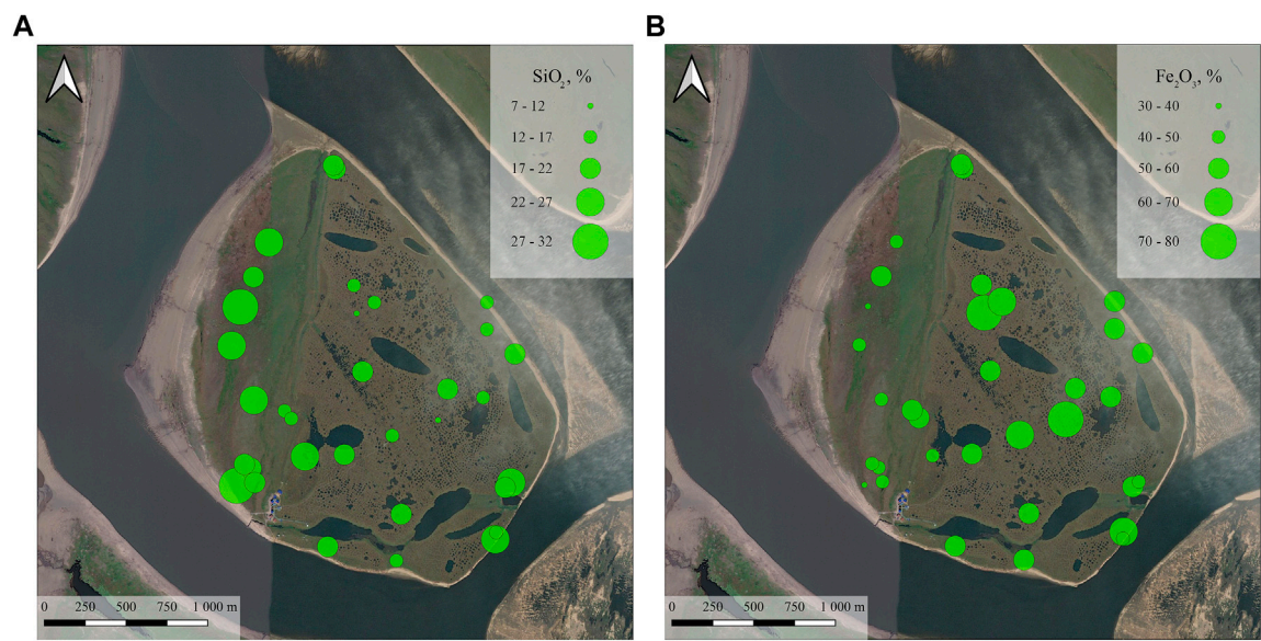
FIGURE 6 Spatial distribution of chemical compounds in study soils. (A) \text{SiO}_2 ; (B) \text{Fe}_2\text{O}_3 .
