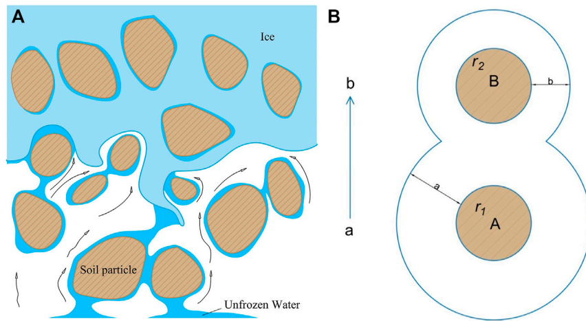
FIGURE 3 | A schematic diagram of film water migration: (A) the direction of film water migration; (B) the principle of film water migration around soil particles (i.e., A and B are soil particles with equal radius, a and b are water film thickness ( a > b ), and particle B is closer to the freezing front).
