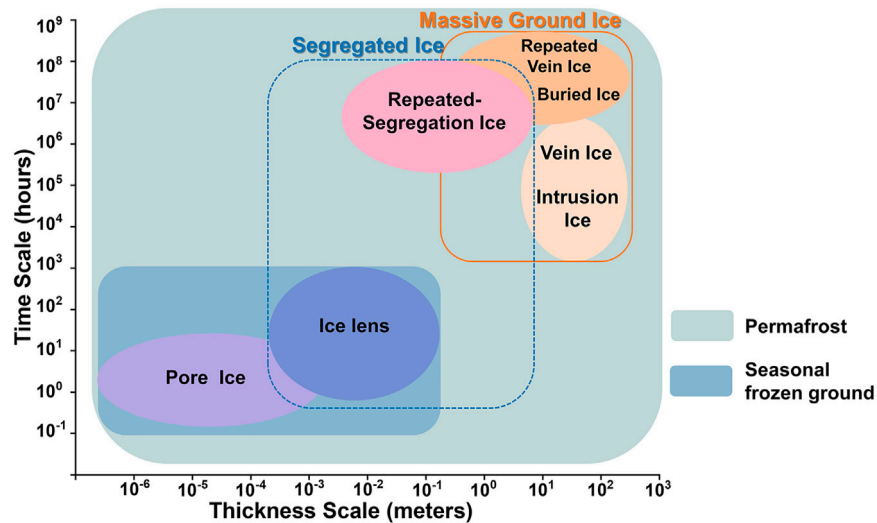
FIGURE 1 | The types of ice in frozen soil range from the pore size to the massive ground ice size at the spatial scale, and their formation ranges from sub-daily to centennial at the temporal scale. The study focuses on the segregated ice and water migration with medium and minor scales (blue dotted line), which exist in permafrost and seasonally frozen ground.
