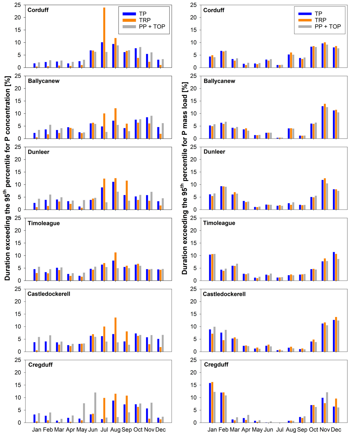
FIGURE 4 Duration of time per month (percent) exceeding the 95 th PCTL of P concentrations (left) and P mass loads (right) for the six study catchments. The data is based on hourly averages of concentrations and hourly totals of mass loads for 10 years (1st October 2010 to 30th September 2020).
