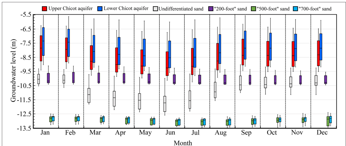
FIGURE 14 | Intra-annual monthly groundwater level variation for different sands in the Chicot aquifer system from 2005 to 2014. The groundwater level datum is NAVD 88.
