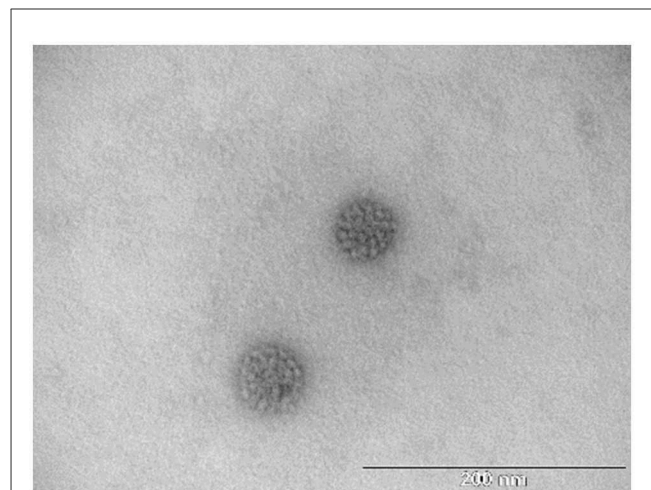
FIGURE 3 TEM micrographs of the isolated BPV1 L1 VLPs. Scale bar = 200 nm.
