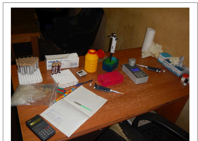
FIGURE 2 | Field set-up to perform the Fluorescence Polarization Assay (FPA) in a slaughterhouse in Abidjan, Côte d'Ivoire.
