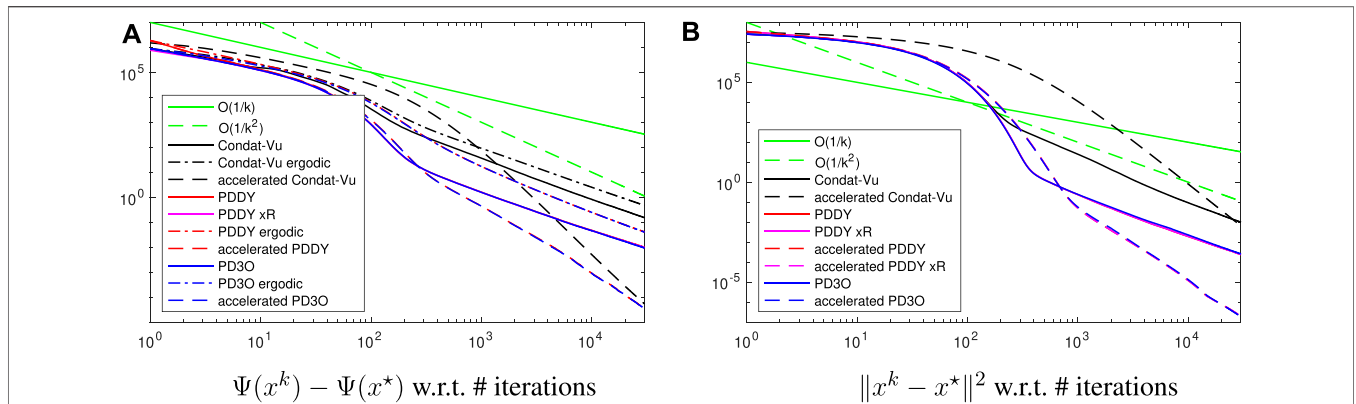
FIGURE 1 | Convergence error, in log-log scale, for the experiment of image deblurring regularized with the total variation, see Section 4.1 for details.
