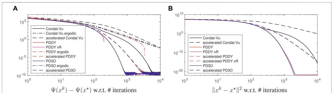
FIGURE 2 | Convergence error, in log-log scale, for the experiment of image deblurring regularized with the smooth Huber-total-variation, so that linear convergence occurs, see Section 4.2 for details.
