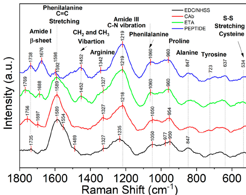
FIGURE 3 Raman spectra in the Fingerprint region (1800–500 \text{cm}^{-1} ) for each functionalization step: (black) MBs-COOH activated with EDC-NHSS incubation; (red) MBs-COOH-CAb; (green) MBs-COOH-CAb stabilized with ETA and (blue) MBs-COOH-CAb@peptide-DAb-HRP.
