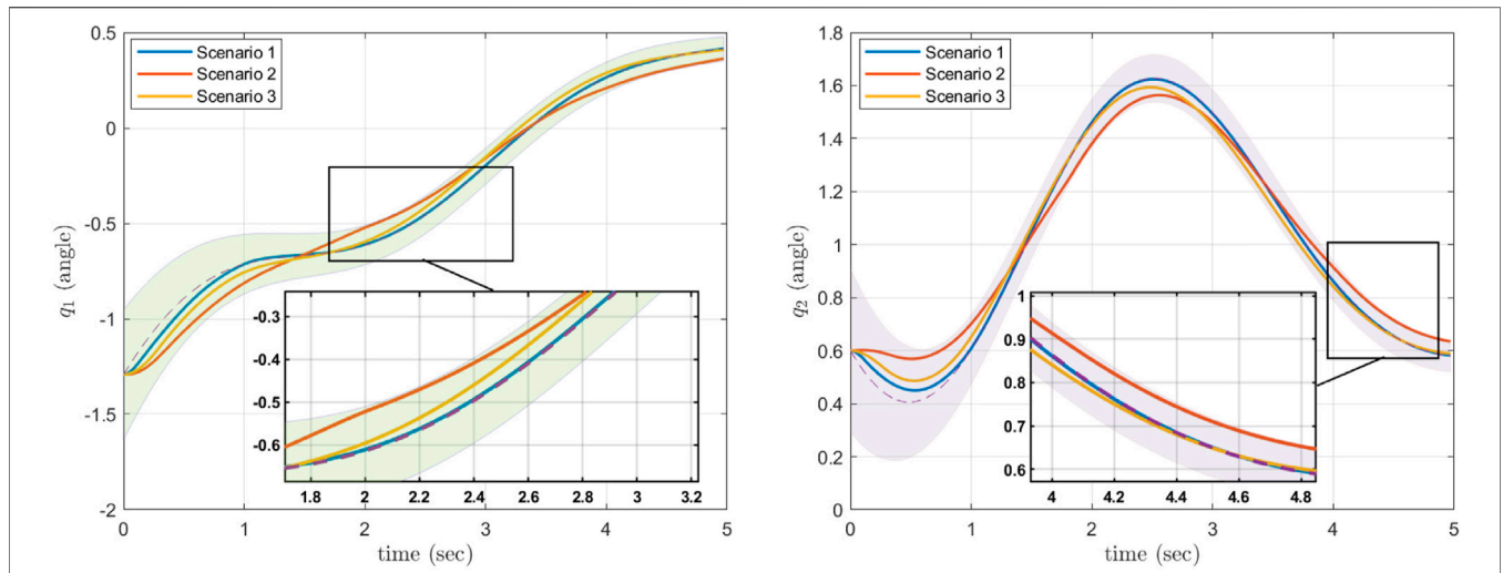
FIGURE 5 | The results of the CLF/CBF-based ProMP controller for the first joint (left) and second joint (right). The safe region of \mu_i \pm \sigma_i, i \in \{1, 2\} is shown as a filled “tube.” The control results in different trajectories for distinct values of the weight \rho_{sc_i} , however all trajectories remain safe. Copyright 2021 IEEE. Reprinted, with permission, from Davoodi et al., 2021.
