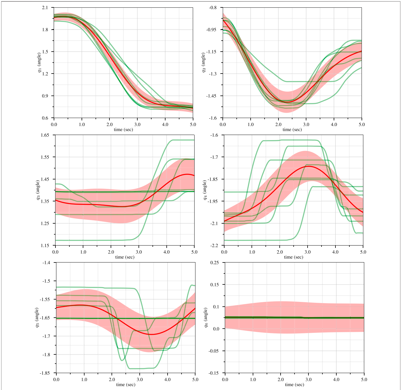
FIGURE 12 | The UR5e robot joint trajectories recorded from the human demonstration of the pick-and-place task are shown in green, while the ProMP mean trajectory and one standard deviation of the ProMP are colored red and light red, respectively.
