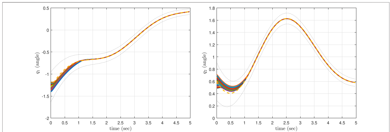
FIGURE 6 | The results of the CLF/CBF-based ProMP controller with more priority given to the CLF than the CBF for the first joint (left) and second joint (right).
