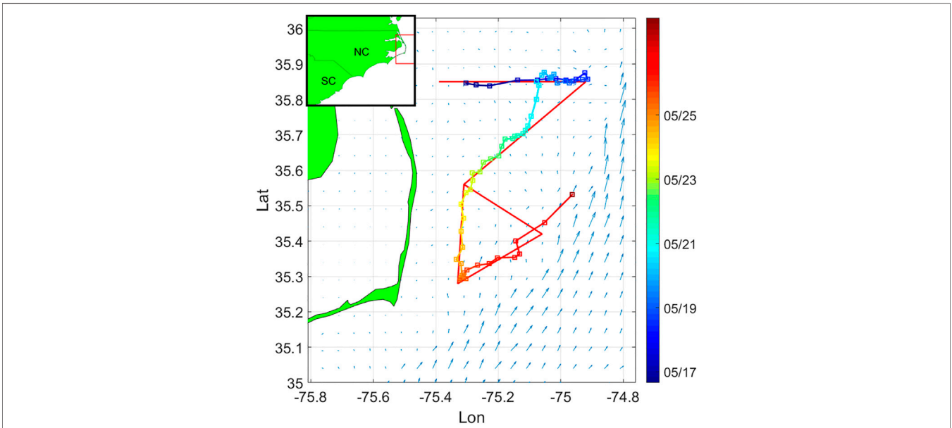
FIGURE 3 | Survey domain near Cape Hatteras. The curve represents glider trajectory during the first PEACH deployment. The red line path is the pre-assigned sampling pattern. Squares denote the glider surfacing positions along trajectory, and color of the trajectory depicts timestamps. The arrows represent the NCOM-predicted flow field at the starting time of the deployment.
