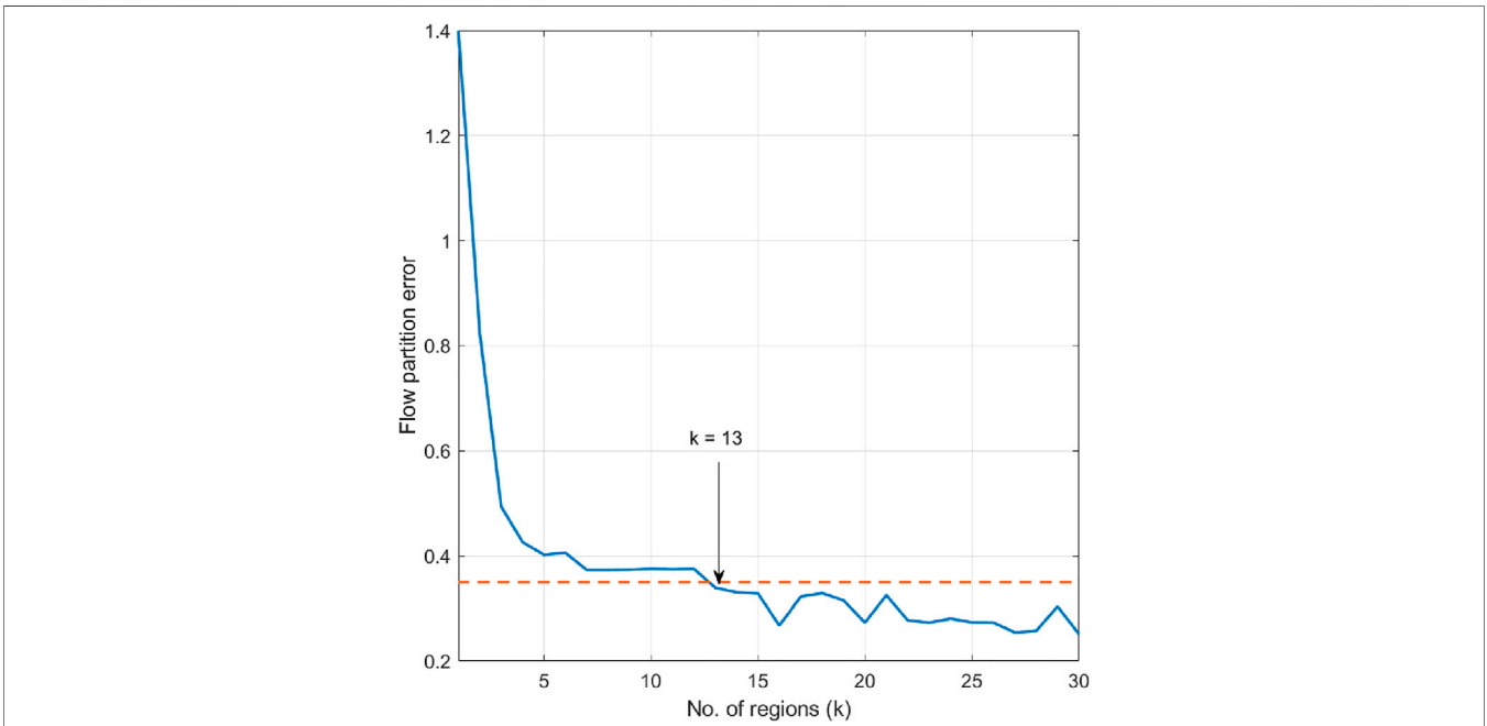
FIGURE 4 | Flow partition error when the number of cells is set as k = 1, \dots, 30 .
