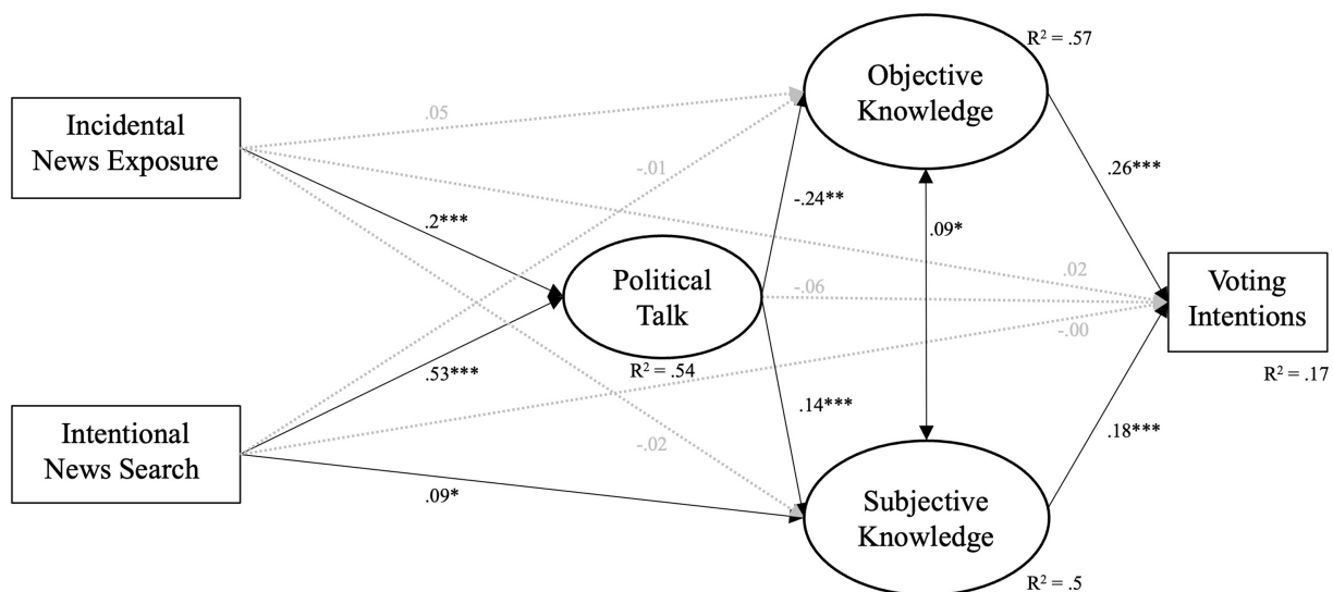
FIGURE 2 Model 2. Model Fit: c2(286)=912.761 p < 0.001, c2/df=3.191, CFI=0.95, RMSEA=0.04 (90% CI: 0.039, 0.045), SRMR=0.04; p < 0.05 (*), p < 0.01 (**), p < 0.001 (***) ; controlled for age, gender, education, and political interest. Full lines indicate significant direct associations, dotted lines indicate non-significant association.
