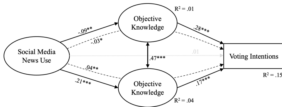
FIGURE 1 Model 1. Model fit: \chi^2(270) = 366.55, p < 0.001, \chi^2/df = 1.75, CFI = 0.98, RMSEA = 0.03 (90% CI: 0.02, 0.03), SRMR = 0.03; p < 0.05 (*), p < 0.01 (**), p < 0.001 (***) ; Full lines indicate significant direct associations, dashed lines indicate indirect significant associations, dotted lines indicate non-significant association.
