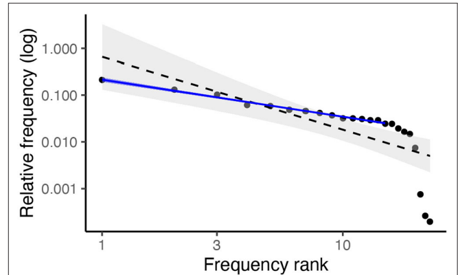
FIGURE 2 | Log-log plot of frequencies vs. frequency ranks in Walmajarri. When a linear model is fitted to the full distribution (dashed black), high and low frequency segments are overestimated and mid-rank segments are underestimated. When lowest-frequency segments are removed from the model (solid blue), the model appears to fit well.
