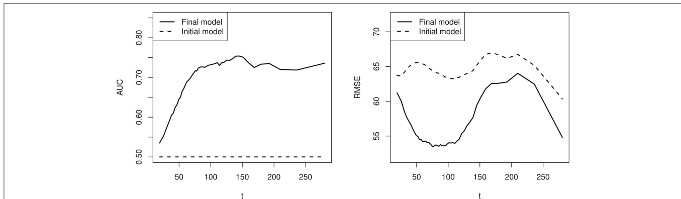
FIGURE 5 | A comparison of prediction accuracy between the model selected by cross validation and a baseline model without using individual specific event history.
