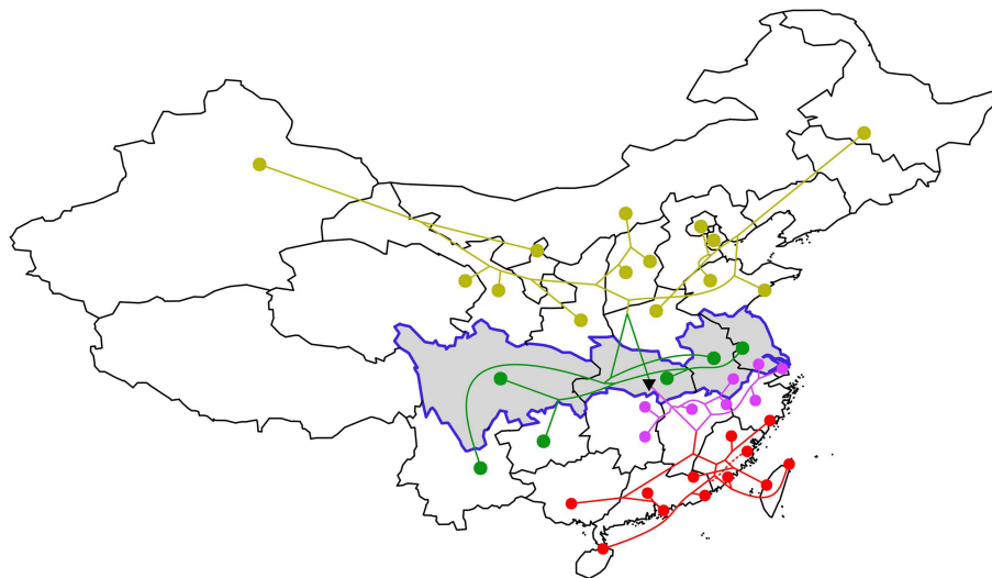
FIGURE 1 | A tree of historical relationships between language varieties constructed from hierarchical clustering of similarities in vocabulary. Provinces on the “rice–wheat” border are highlighted in gray (provinces south of the border produce more rice). The black triangle
