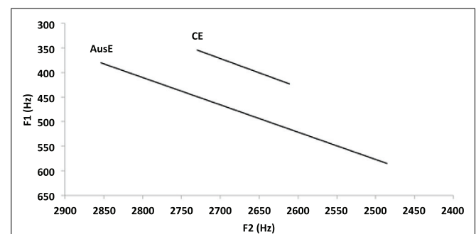
FIGURE 4 | Average spectral change for the vowel /i/ in the ten familiarization tokens of DEET for the two accents. The accent label and the end of each line are plotted at the average formant frequency (across tokens) at 75% of the vowel duration, and each line originates at the average formant frequency at 25% of the vowel duration. There was a larger movement of the formants across the 25 and 75% points of the vowels in the AusE than in CE.
