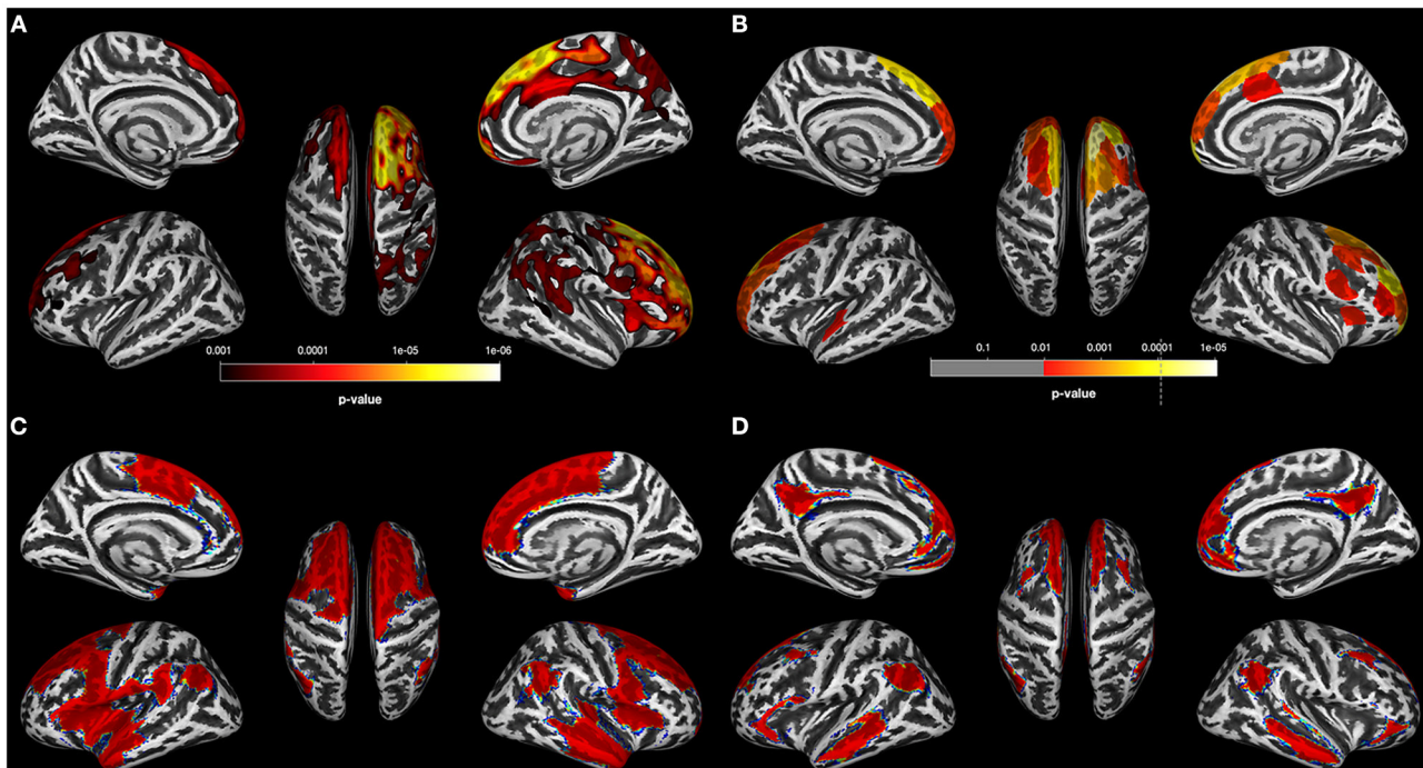
FIGURE 1 | Results for AUD individuals (A) . Results of the data-driven vertex-wise cortical thickness (CT) analysis—controls have significantly higher CT values than alcohol use disorder individuals (AUD) at p = 0.001 FWE corr. (TFCE). (B) Results of the data-driven ROI analysis with the Schaefer Atlas (48) (200 parcels) colored are ROIs for which controls have significantly higher mean CT values than AUD at p = 0.01 FDR corr.; (C) CT covariance results highlighted with red color all Schaefer ROIs with which the two ROIs corresponding to the two peak vertices of the most significant clusters in (A) show significant positive correlations at p < 0.05 . (D) Result of the Neurosynth seed correlation analysis (thresholded at r > 0.2 ) with resting-state data of 1,000 healthy participants with the MNI coordinates of the two peak vertices of the most significant clusters in (A) as seeds.
