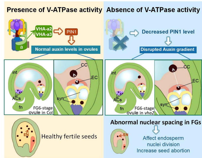
FIGURE 8 Schematic diagram of the role of V-ATPase on FGs and later endosperm development. fn funiculus, syn synergid cell, EC egg cell, CC central cell, ACs antipodal cells, int integuments (inner and outer).
