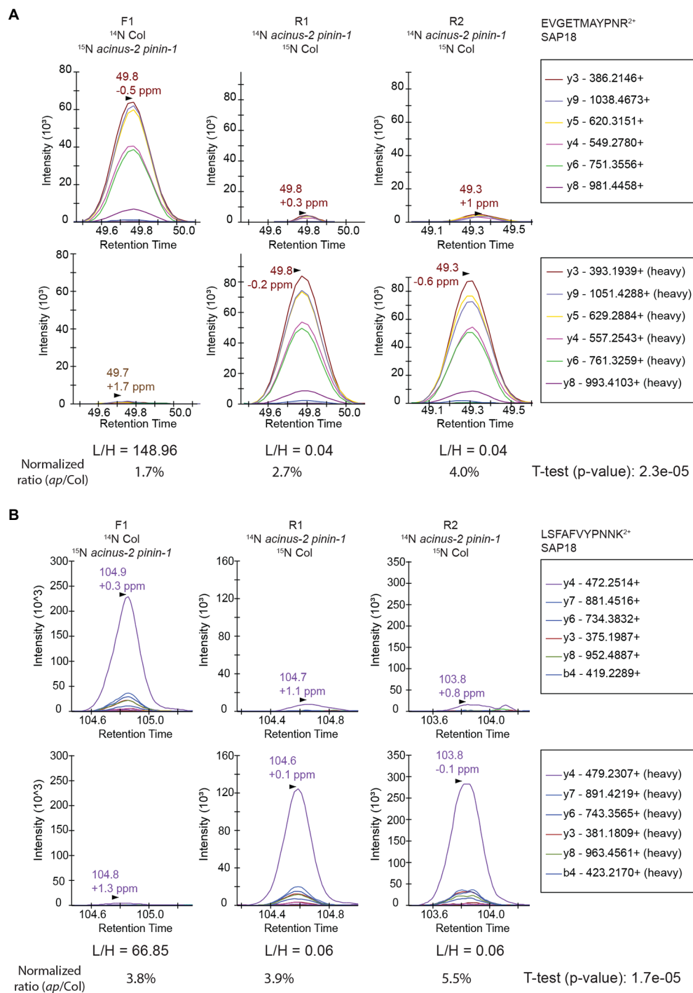
FIGURE 6 | Targeted quantification using PRM on SAP18 proteins provides unambiguous quantification results. The targeted quantifications in three samples gave consistent results showing SAP18 was dramatically reduced in acinus-2 pinin-1 mutant after normalization to TUB2. The light and heavy peptides gave a similar pattern of fragmentation. The peptides are quantified using area under the curve (AUC). (A) PRM results from peptide “EVGETMAYPNR” confirm the heavy matching peaks in Figure 4C is indeed from a co-eluting ^{14}\text{N} labeled peptide; (B) PRM results from peptide “LSFAFVYPNNK” confirm the matching ^{14}\text{N} peak in MS 1 Figure 4E from DDA data is indeed contaminated with overlapping peaks.
