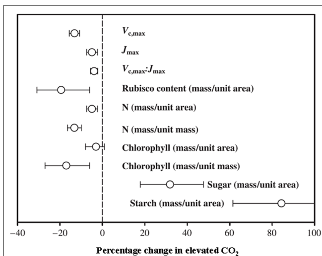
FIGURE 1 | Mean response of maximum carboxylation rate ( V_{c,max} ), maximum rate of electron transport ( J_{max} ), ratio of V_{c,max} : J_{max} , and Rubisco, N, chlorophyll, sugar and starch contents. Rubisco, sugar and starch contents reported on area basis. N and chlorophyll contents reported on both area and mass basis at 95% confidence level. Number of species, FACE experiments and individual observations for each response are given in Ainsworth and Long (2005). LAI, leaf area index; DMP, above ground dry matter production (Reproduced with permission).
