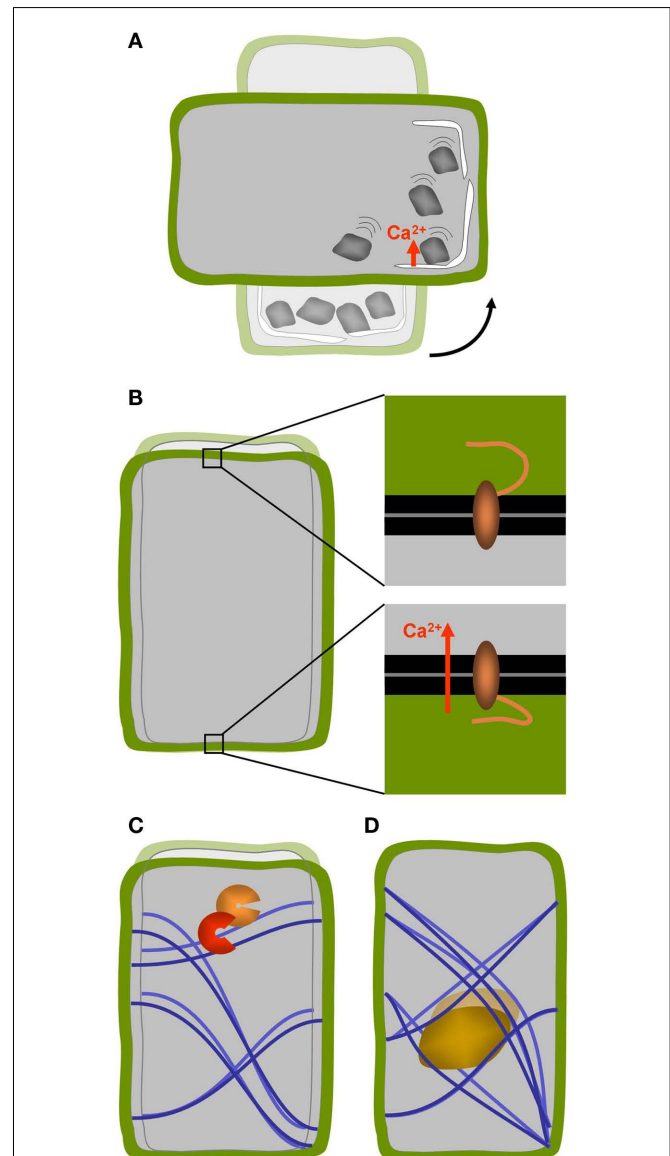
FIGURE 2 | Concepts of cellular gravisensing in plants. (A) In statolith-based gravisensing the sedimentation or change of position of intracellular organelles with higher density triggers a signal most likely based on a change in trans-membrane ion fluxes. (B) According to the gravitational pressure model the weight of the protoplast causes the forces acting on the membrane–cell wall connections at the upper and lower sides of the cells to be different. (C) The tensegrity model predicts that cellular distortion due to a change in g -force affects the pre-stress in the cytoskeletal array of the cell which in turn changes biochemical activities. (D) A variation of the tensegrity model is based on a change in cytoskeletal pre-stress being caused by the weight of heavy organelles that are tethered to the cytoskeletal filaments such as the nucleus.
