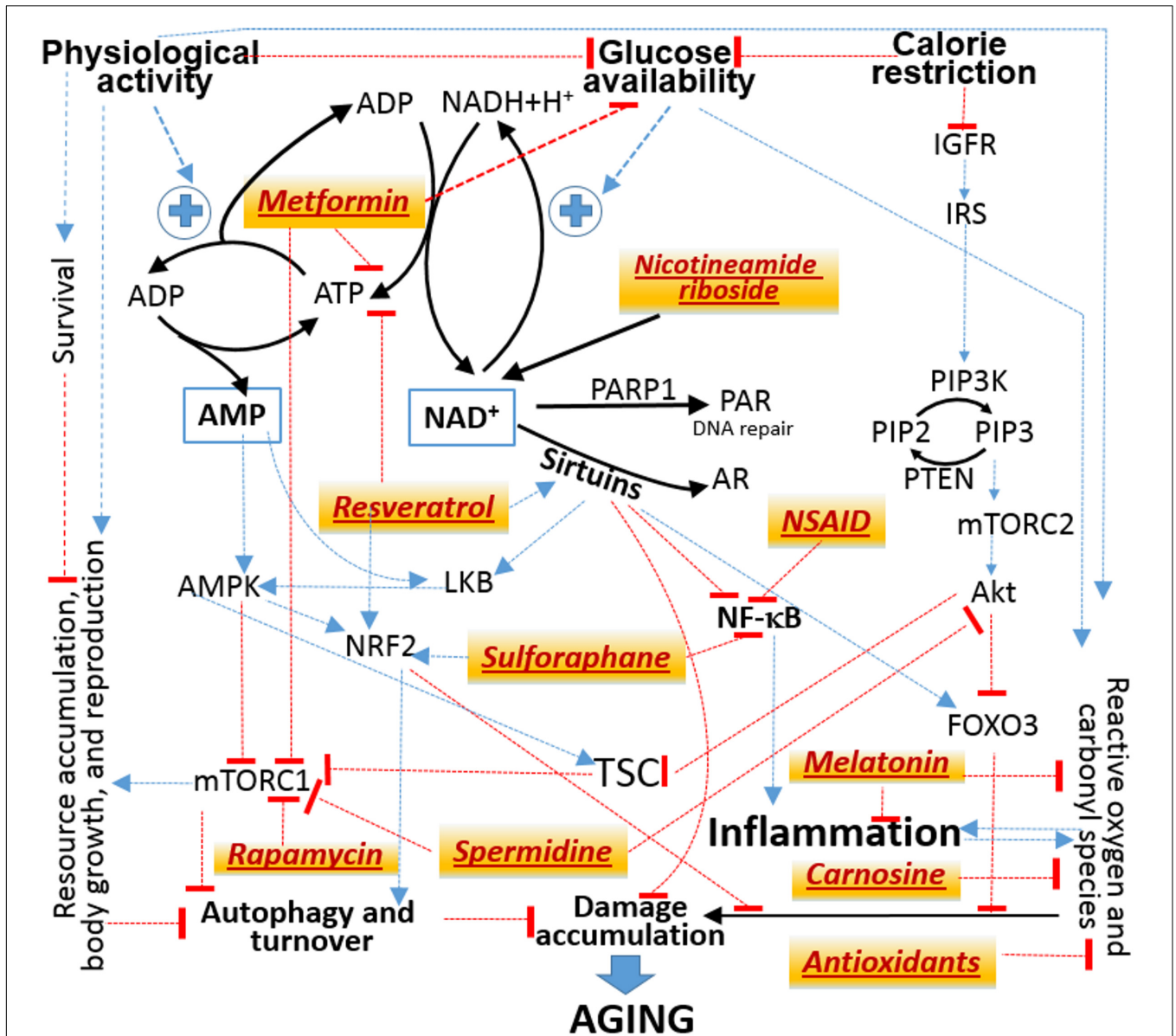
FIGURE 3 | Attribution of the molecular targets of drugs suggested to treat both aging and COVID-19 (tan background) to signaling pathways from the availability of nutritional calories embodied in glucose to the physiological responses that allocate available resources between storage, growth and reproduction vs prevention and repair of molecular damage. Black solid lines designate mass transfer. Thin lines designate influences without specifying their mechanisms. Some may involve additional steps and intermediates, which are not shown. Blue arrows stand for activation or enhancement. Red bricks stand for inhibition or suppression. Abbreviations are explained in the main text.
