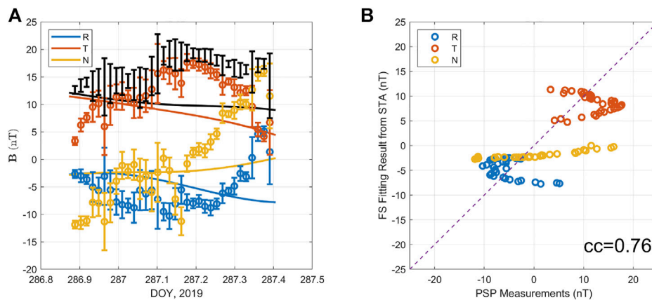
FIGURE 7 (A) The comparison between the FS model output (smooth curves) based on the optimal fitting to STA data only and the actual measurements (errorbars), along the PSP spacecraft path, as illustrated in Figure 6. (B) The corresponding component-wise correlation plot between the two sets of data, yielding an overall correlation coefficient cc = 0.76 . The diagonal dashed line indicates the one-to-one line. The corresponding correlation coefficients for each magnetic field component in the RTN coordinates are -0.46 , -0.14 , and 0.91 , respectively.
