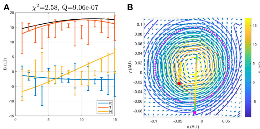
FIGURE 8 (A) The two-spacecraft (STA-PSP) optimization result of the magnetic field components and magnitude (black curve) for the STA data interval. Format is the same as Figure 4. (B) One cross section for the optimal FS model result based on the two-spacecraft (STA-PSP) optimization (with a = 0.049 AU). Format is the same as Figure 5.
