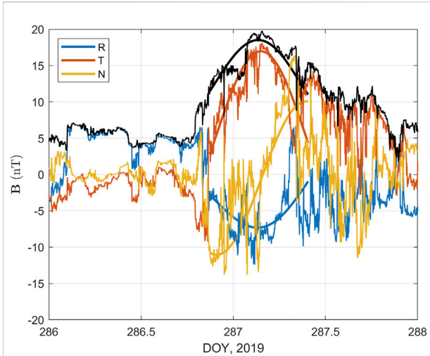
FIGURE 3 The corresponding magnetic field measurements including the magnitude (black) from PSP in the RTN coordinates during day of year, DOY 286 (October 13), and DOY 288, 2019. The smooth curves are the FS model output from the two-spacecraft optimization presented in Modeling and optimization of the ICME magnetic structure .
