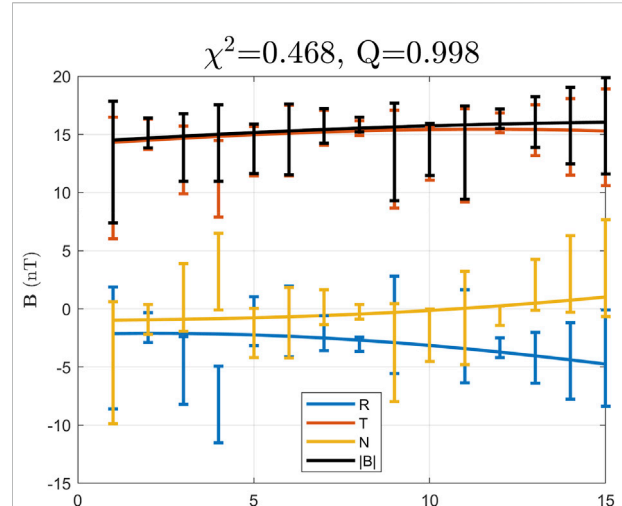
FIGURE 4 The optimal FS model fitting result (smooth curves) to the STA data (errorbars) only for the interval marked in Figure 2 . The corresponding minimum reduced \chi^2 and Q values are denoted on top. The horizontal axis indicates the indices of the data arrays (15 data points each).
