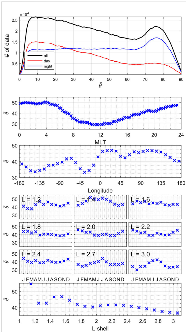
FIGURE 8 (first panel) Distributions of the wave normal angle ( \bar{\theta} ) (in ^{\circ} ) at (red) day (6–17 MLT), (blue) night (18–5 MLT), (black) all times. Wave normal angle is plotted versus (second panel) MLT and (third panel) longitude. The day/night differences appear clearly but not the continental dependence. (fourth panel) Monthly and (fifth panel) total average of wave normal angle versus L-shell. No simple seasonal dependence is found.
