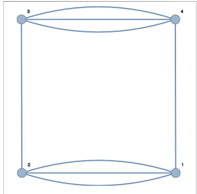
FIGURE 2 | The quartic tensorial bubble interaction B_{41} .
