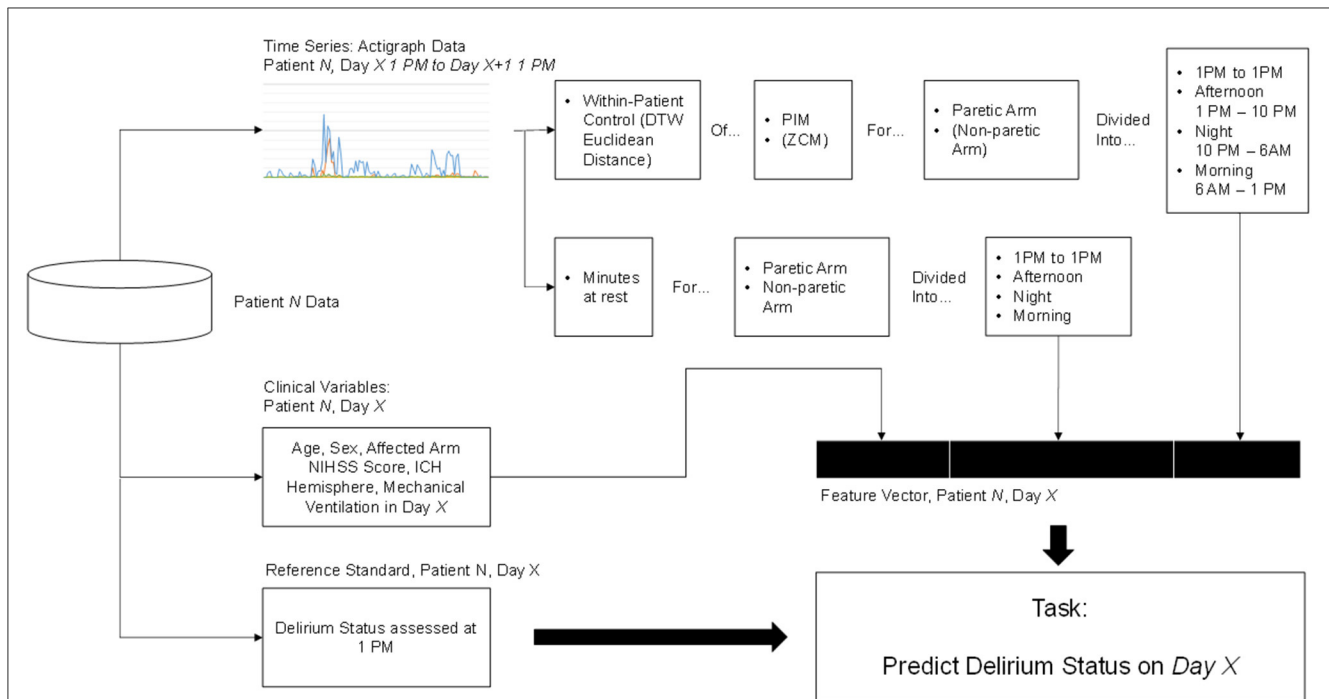
FIGURE 1 Feature extraction and classification process. Elements in parentheses were initially explored but ultimately discarded because they did not contribute to higher prediction accuracy.
