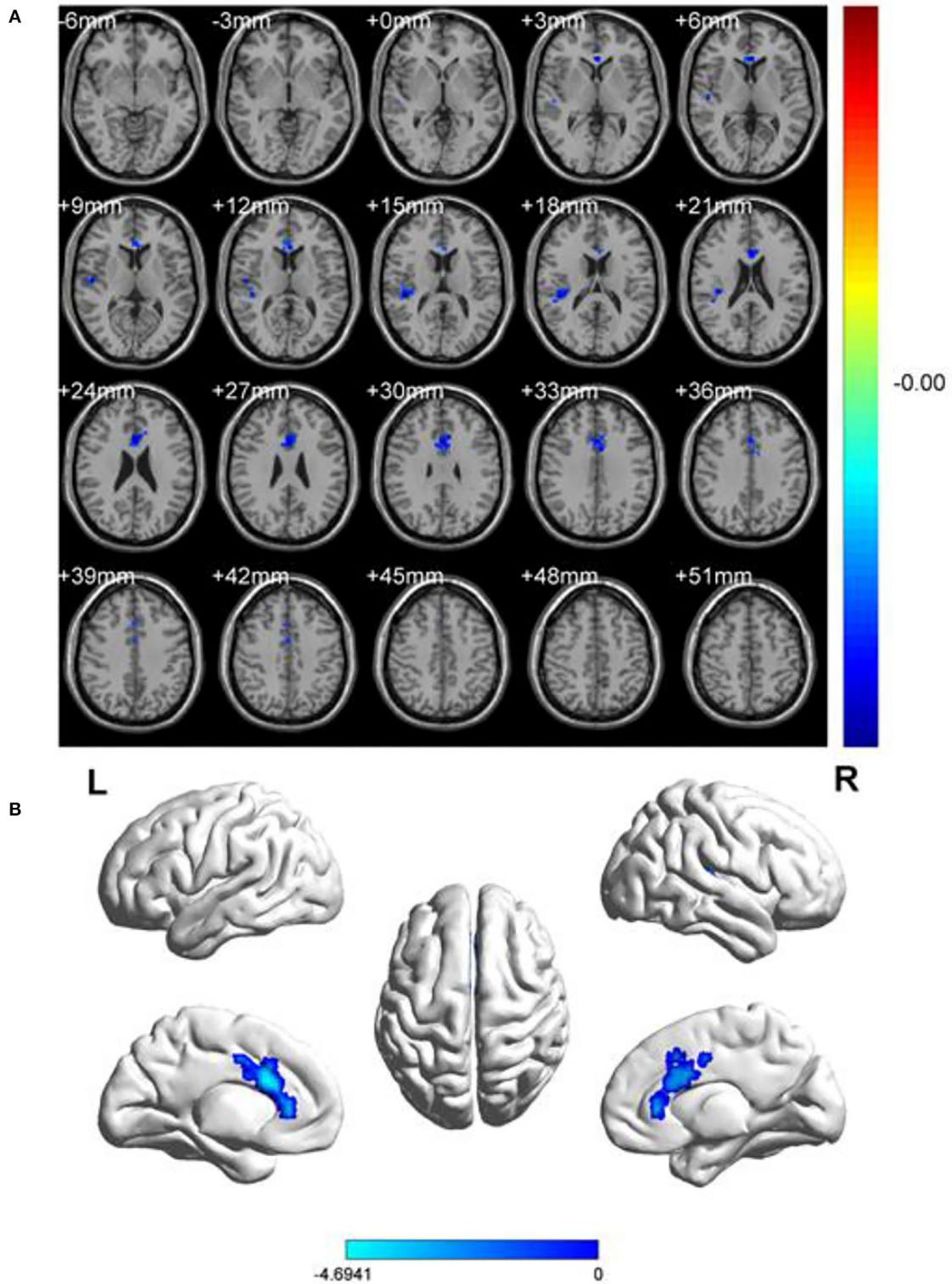
FIGURE 1 | Spontaneous brain activities of and healthy controls. (A) Different fALFF areas in patients with OF. (B) The blue areas represented lower fALFF values. L, left; R, right.
