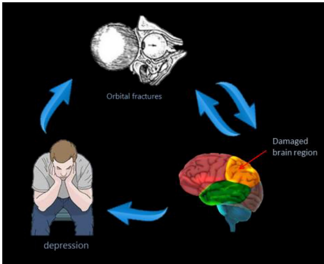
FIGURE 5 | The correlations between average fALFF signal values and clinical manifestation of patients with OF. The patients with OF have lower fALFF values, and they are more likely to develop depressive symptoms. OF, orbital fractures.
