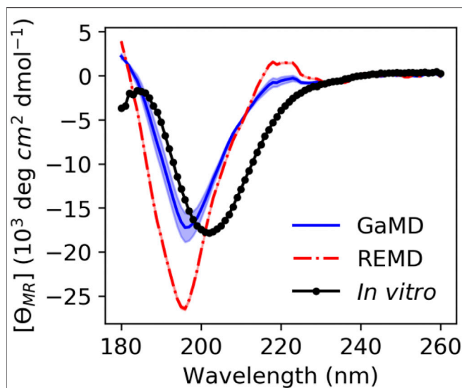
FIGURE 7 | ArkA in vitro CD spectrum (black solid line with data points as circles) compared to the calculated theoretical CD spectrum based on the ArkA GaMD (solid blue line) and REMD (dashed red line) ensembles. The theoretical spectra were calculated using SESCO (Nagy et al., 2019) and scaled by a factor of 0.51. The shaded region represents the standard deviation over all independent simulations for each system (the REMD shaded region is the same width as the line).
