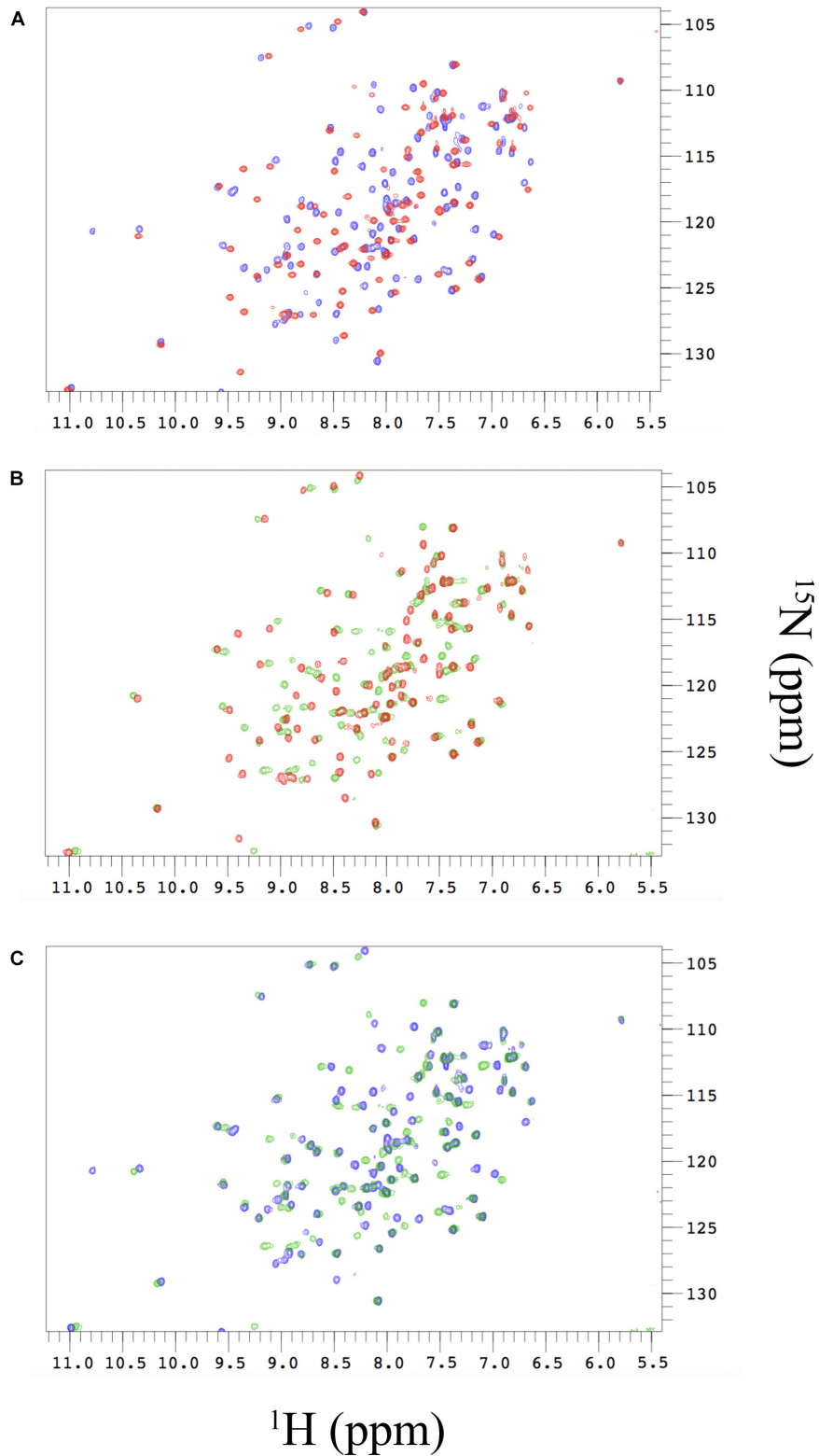
FIGURE 4 | (A) Changes in the ^1\text{H} - ^{15}\text{N} -HSQC spectra of free N-SH2 (red peaks) and N-SH2 in complex with Gab2 448-460 (blue peaks). (B) Changes in the ^1\text{H} - ^{15}\text{N} -HSQC spectra of free N-SH2 (red peaks) and N-SH2 in complex with Gab2 448-460 M457A (green peaks). (C) Comparison of ^1\text{H} - ^{15}\text{N} -HSQC spectra of the bound states of N-SH2 with the two variants of Gab2 peptide. The analysis reveals that the M457A mutation in the ligand modulates the plasticity of N-SH2 in the complex.
