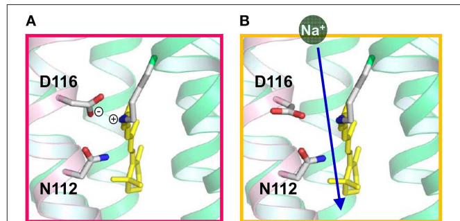
FIGURE 12 | Proposed local structures of KR2 in the dark (A) and in the M intermediate (B), suggested from crystal structures of KR2 at different pHs.
