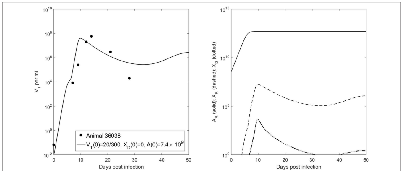
FIGURE 5 | (Left) V_T given by (4) vs. data; (Right) Free antibody (solid lines), recipient immune complexes (dashed lines) and donor immune complexes (dotted lines) for V(0) = 20/300 vRNA copies per ml, X_D(0) = 0 vRNA copies per ml and A_D(0) = 7.4 \times 10^9 molecules per ml.
