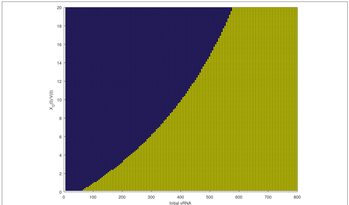
FIGURE 4 | Asymptotic behavior for the V_T solutions of (4) for median parameters in Table 3 as the initial vRNA and X_D(0)/V(0) are varied. The blue region (left of the curve) corresponds to extinction asymptotic concentrations V_T = 0 copies per ml. The yellow region (right of the curve) corresponds to persistence asymptotic concentrations V_T = 6.9 \times 10^6 copies per ml.
