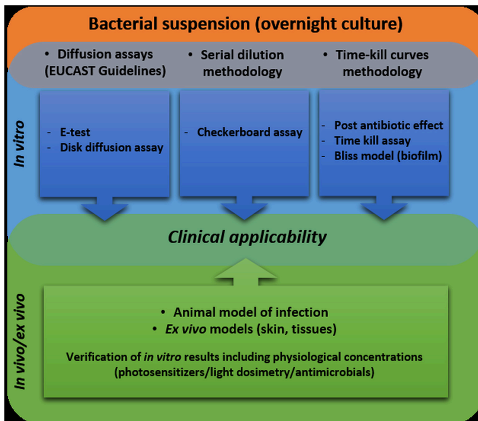
FIGURE 2 | Workflow including recommended methodologies for testing the synergy between antimicrobial photodynamic inactivation and antibiotics.
