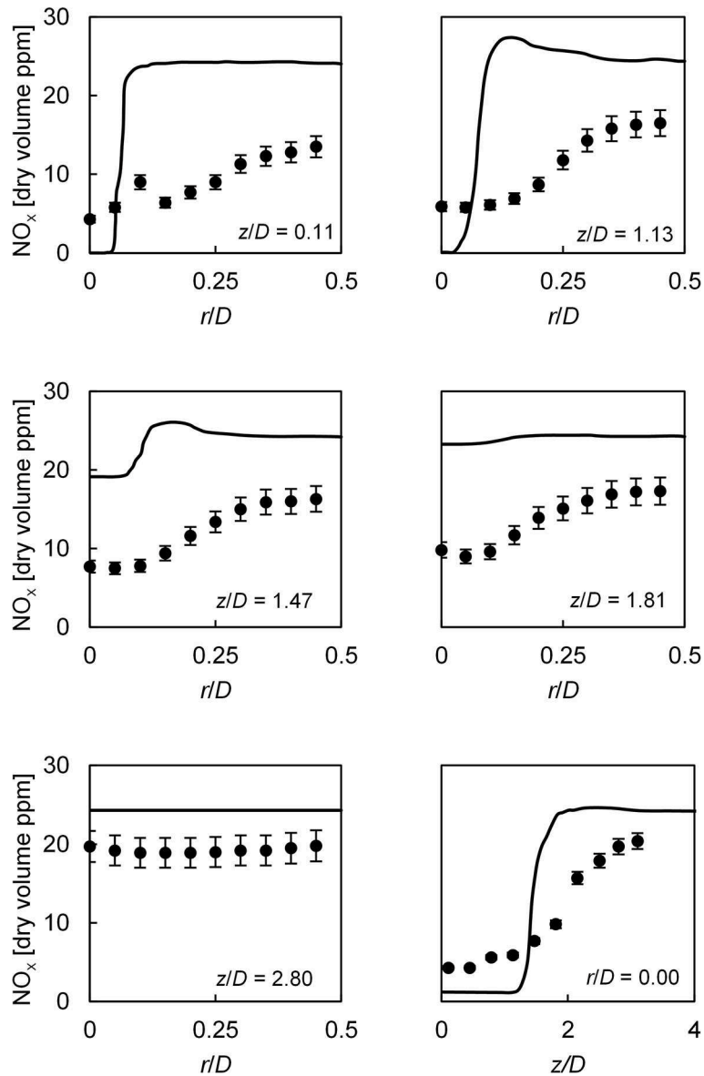
FIGURE 13 | NO x values at selected local profiles. Comparison between experimental data and AGNES results obtained using an FGM simulation as input, GRI 2.11 and T, velocity direction, Y H2O , Y CH4 , and Y O2 as clustering criteria for condition b ( \phi \cong 0.77 ).
