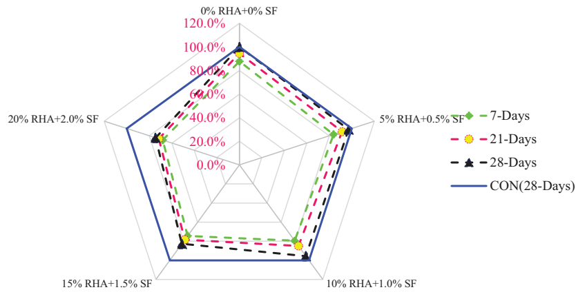
FIGURE 5 | Relative analysis of compressive strength (with steel fibers and superplasticizer).
