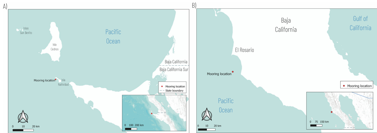
FIGURE 4 Maps showing the mooring locations at (A) Isla Natividad and (B) El Rosario, indicated by red dots.
