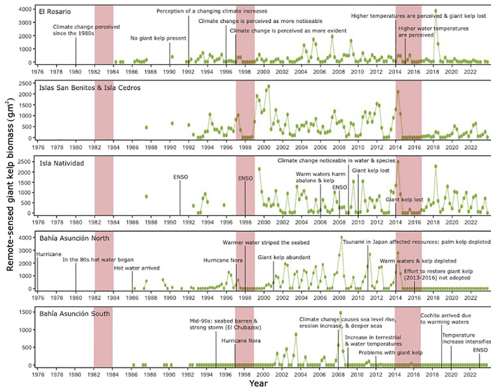
FIGURE 5 Time series of canopy kelp biomass ( \text{g}/\text{m}^2 ) detected in each quarter of the year, along with information about events impacting kelp biomass for each of the five cooperatives in Baja California, Mexico. The pink shaded polygons represent years with the strongest warming events (1982–1983 ENSO, 1997–1998 ENSO, and 2014–2016 “Blob” + ENSO). The text includes ethnographic records related to environmental events and kelp dynamics for each community.
