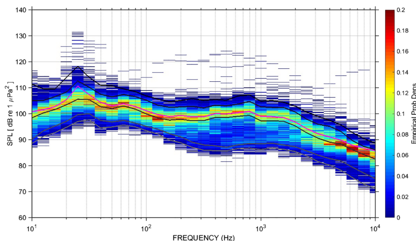
FIGURE 7 Empirical probability density of the median SPL power spectra (SPL50p, dB re 1μPa 2 ) calculated from acoustic data of FA-01 mooring line measured in the time interval of 09/April/2019 to 13/November/2019. Magenta line is the average spectrum. Gray lines from below to above represent the 5 th , 25 th , 50 th (median), 75 th , and 95 th percentiles.
