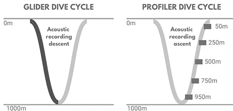
FIGURE 4 Schematic view of glider dive (left panel) and profiler dive (right panel) at PMPAS-BS. The gliders were programmed to activate the PAM during the descent phase and the profilers acquired acoustic data during the ascent phase.
