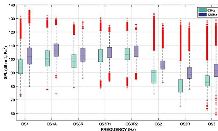
FIGURE 8 Box plots with comparison between OSs for all data (SPL50p, dB re 1 \mu Pa 2 ) in the 1/3 octave filters at frequencies of 63 Hz (green rectangles, left in each pair of rectangles) and 125 Hz (blue rectangles, right).
