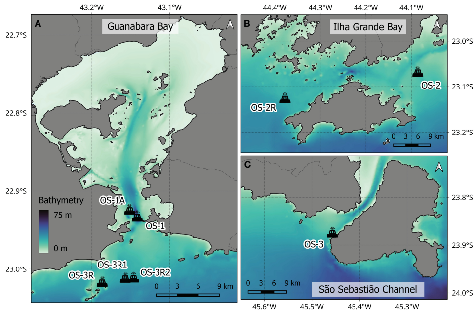
FIGURE 3 Detailed maps of the coastal O/Ss positions in Guanabara Bay and surroundings of the Natural Monument Cagarras Archipelago Islands (A), Ilha Grande Bay (B), and São Sebastião Channel (C). The background color scale indicates water depth.
