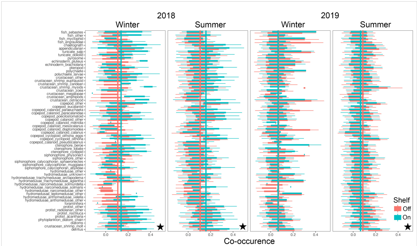
FIGURE 9 Co-occurrence of plankton taxa (y-axis) with all other taxa on the shelf (green) and off the shelf (red) along the Trinidad Head line. Vertical lines indicate taxa averages of co-occurrence as measured by spatial correlations. Stars indicate significant differences between on-, and off-shelf co-occurrence averages using Wilcoxon Rank Sum tests ( p < 0.0001 ). Boxplots show the median, and hinges the first and third quartiles. Whiskers extend from the hinges to the largest value but no further than 1.5 \times interquartile range. Single outlier values have not been included due to adverse effects on figure readability, and do not impact interpretation and calculation of statistics.
