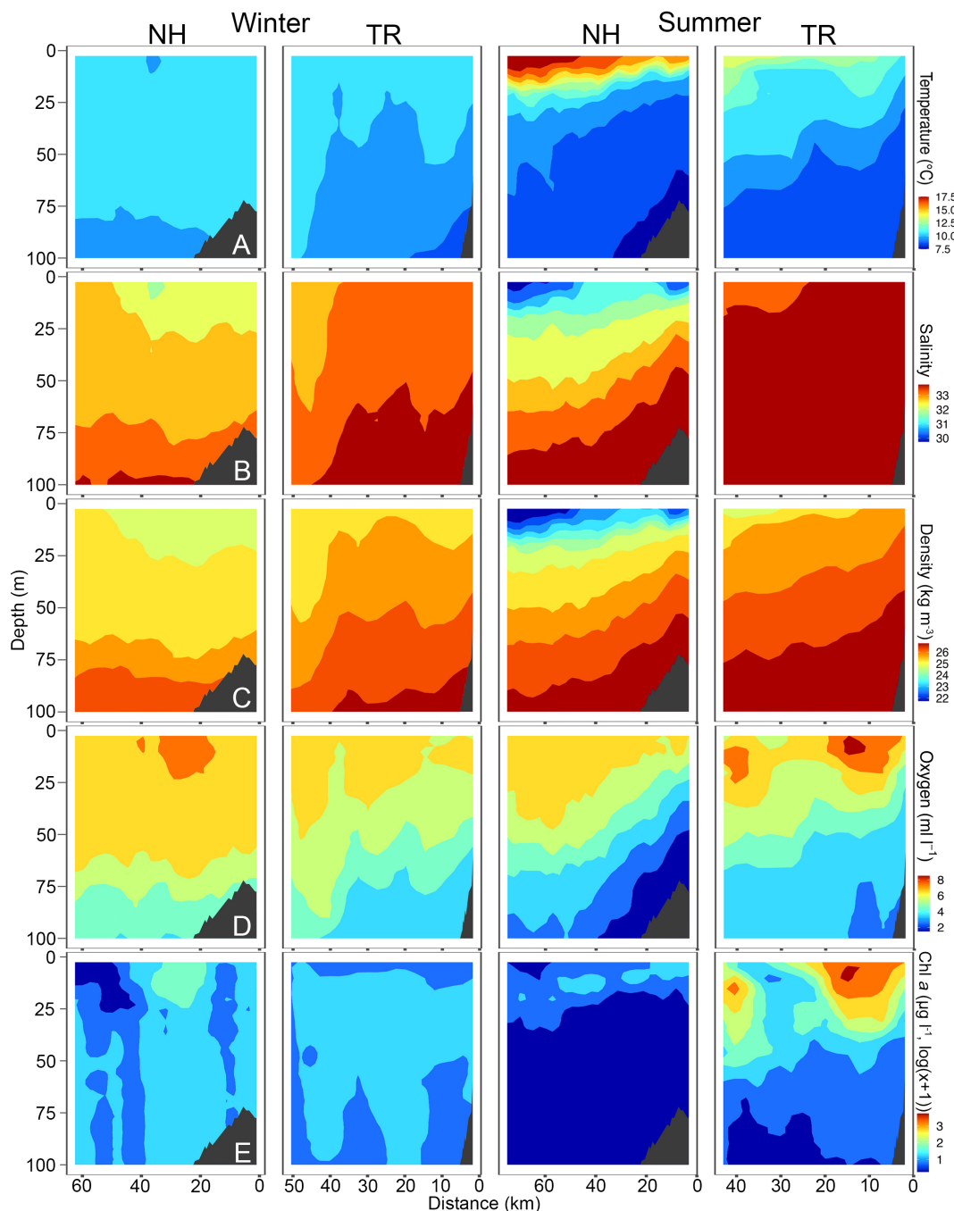
FIGURE 4 Temperature (A), Salinity (B), Density (C), Oxygen (D) and Chlorophyll a (chl a, E) across the Newport Hydrographic (NH) and Trinidad Head (TR) transects in winter and summer 2018. Winter sampling on the NH and TR shown here was carried out February 16 and 21, respectively, while summer sampling was carried out on July 10 and 7, respectively. Note that Chl a is plotted in \log(x+1) due to the values ranging from 0.01 to 45 \mu\text{g l}^{-1} . Shelf indicated in dark grey. Note that x-axes have different lengths.
