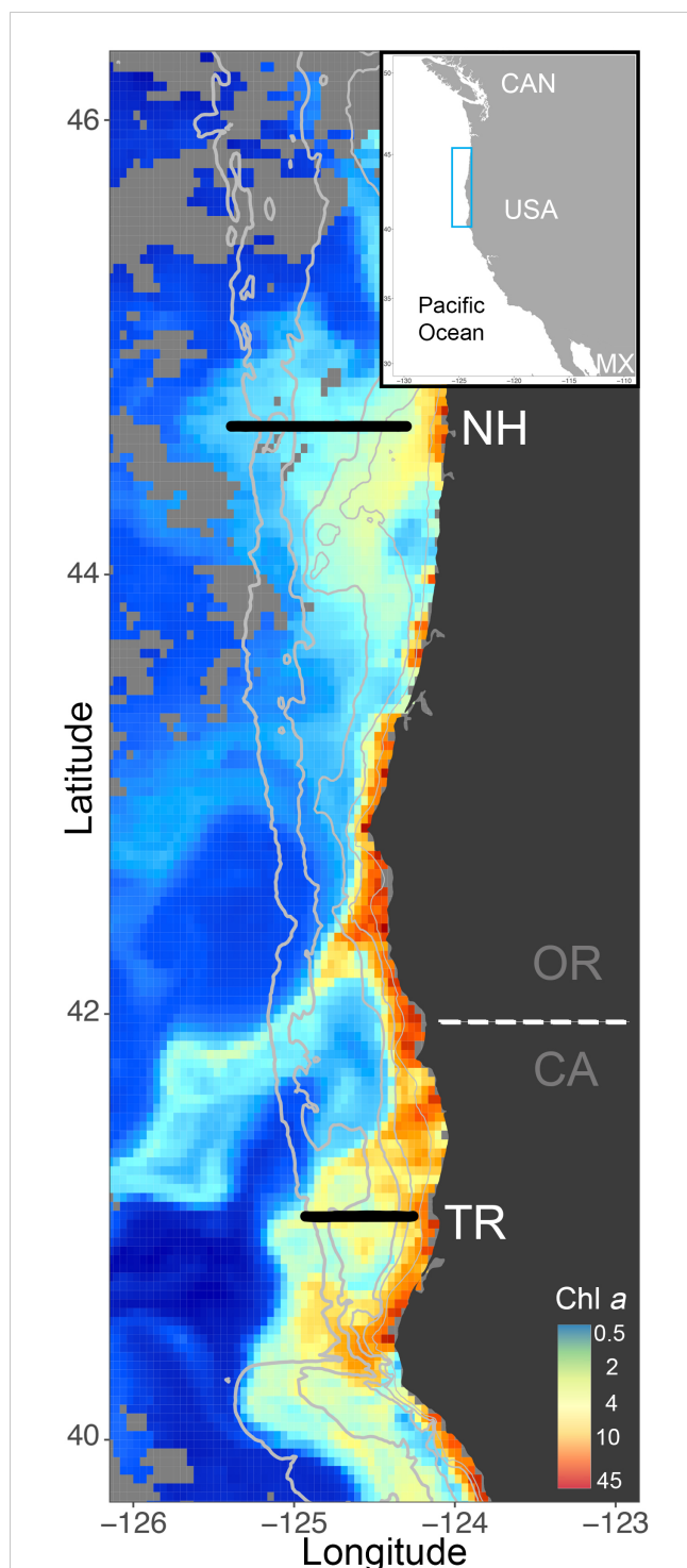
FIGURE 1 ISIIS transects along the Newport Hydrographic (NH) and Trinidad Head (TR) lines (black solid line) in Oregon (OR) and California (CA), respectively, where sampling occurred in winter and summer 2018 and 2019. Chlorophyll a from Aqua Modis ocean color on July 10, 2018 shows the often higher productivity in the northern California part of the Northern California Current, where the shelf is narrower than farther north at the NH Line (depth contours in solid grey lines at 50m, 100m, 200m, 1000m, 2000m). Light grey pixels indicate non-available data from Aqua Modis.
