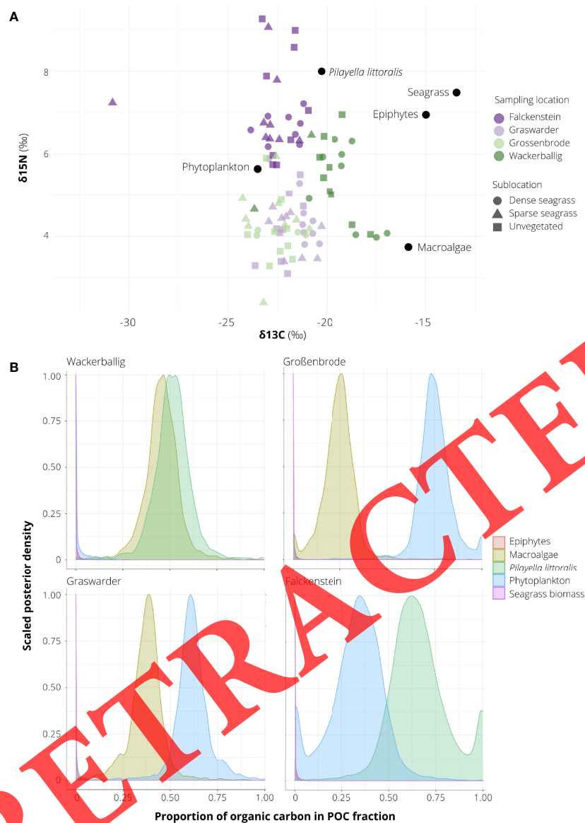
FIGURE 4 \delta^{13}\text{C} and \delta^{15}\text{N} stable isotope signatures (A) and posterior estimates of the proportion of organic carbon ( C_{\text{org}} ) sources (B) of sediments sampled in seagrass-vegetated and unvegetated sublocations off the coasts of Falckenstein (FS), Wackerballig (WB), Großenbrode (GB), Graswarder and (GW) in northern Germany. Sources (black circles) were obtained from Table 1 in Mittermayr et al. (2014) and Table 2 in Maksymowska et al. (2000) .
