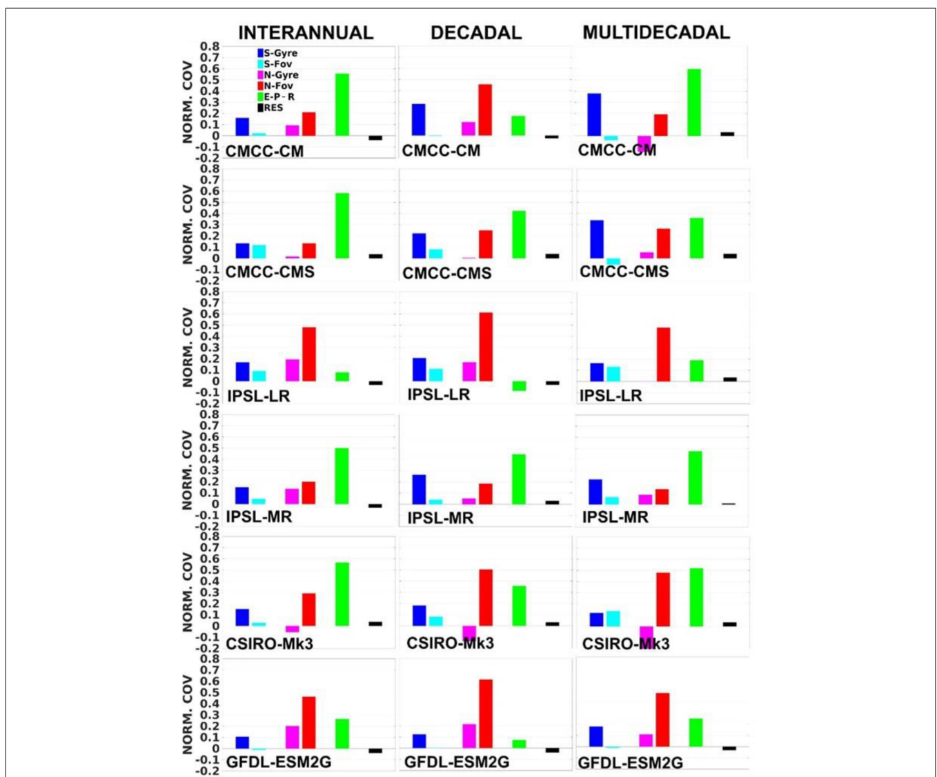
FIGURE 6 | The covariance of each budget term with FWC changes normalised by the variance of FWC changes (Eq. 8, considering the region between 34°S and 40°N). The sum of all normalised covariances, including from the residual term, equals 1. The normalised covariances are evaluated on interannual, decadal, and multidecadal timescales. The prefixes “S-” and “N-” denote southern and northern transports, respectively.
