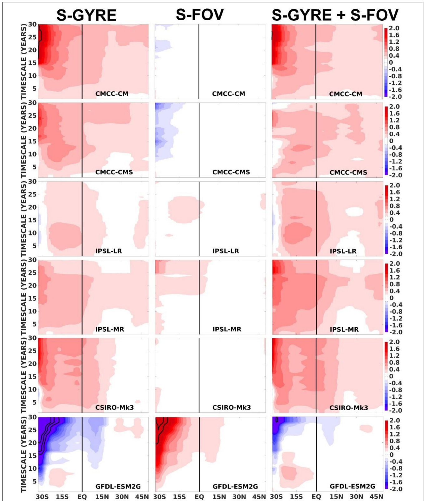
FIGURE 7 | Normalised covariances of the southern F_{gyre} , F_{ov} , and total transports with FWC changes, as in Eq. 8, considering a fixed southern boundary at 34°S and a moving northern boundary from 33°S to 50°N. The spatially varying normalised covariances are evaluated from interannual to multidecadal timescales. The black contours correspond to either negative or positive normalised covariance values of >3 .
