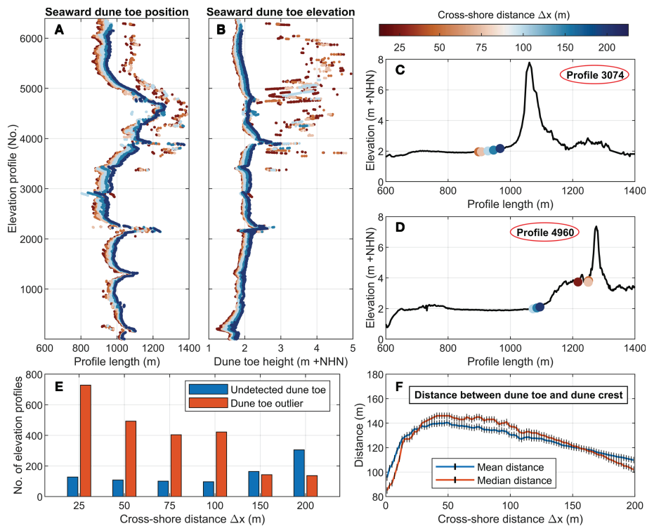
FIGURE 7 Performance evaluation of different specific cross-shore distances \Delta x in 2015 with (A) the positions of all detected seaward dune toes; (B) the heights of all detected seaward dune toes; (C, D) two exemplary elevation profiles; (E) a statistic of undetected and deviant dune toes per \Delta x ; (F) mean and median distances between the seaward dune toe and the dune crest per \Delta x .
