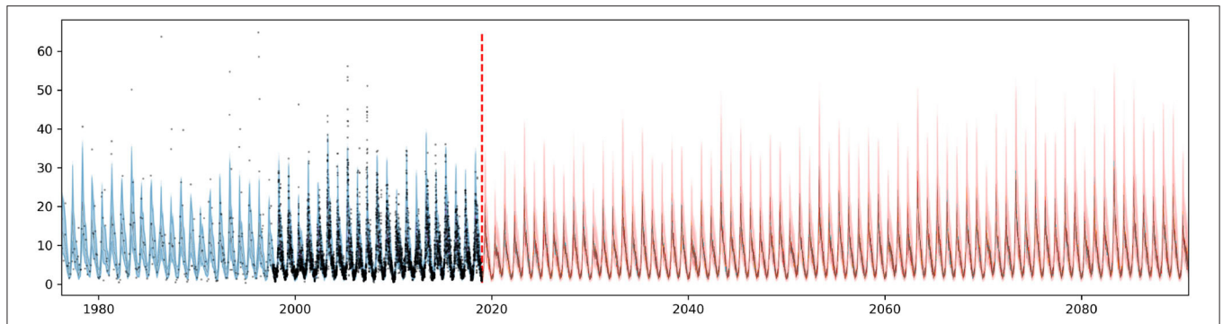
FIGURE 11 | Long term chlorophyll-a concentration time series projection with radiation and temperature explanatory variables from generated climate projections (based on EURO-CORDEX). One hundred and twenty solar radiation and air temperature projection scenarios were used to produce the 120 chlorophyll-a trajectories. Model fit between 1976 and 2018 (blue) and projection between 2019 and 289 (red). Predictive uncertainty in shaded area.
