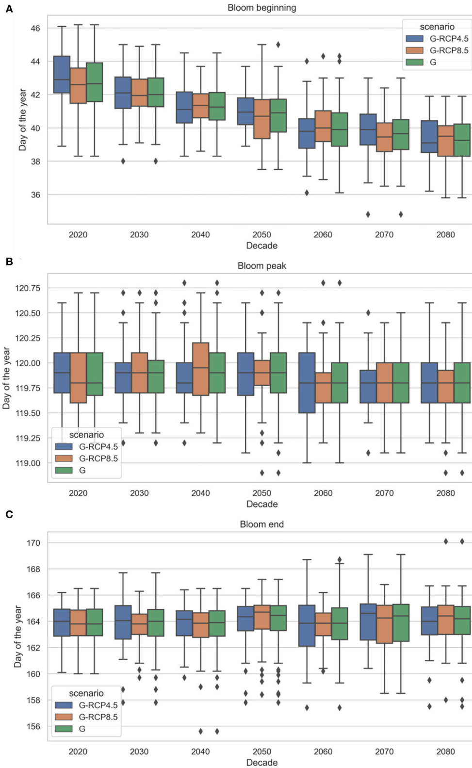
FIGURE 14 | Projected future phytoplankton spring bloom beginning (A) , peak timing (B) , and end (C) under generated (G) radiation and temperature projections (based EURO-CORDEX) (2019–2089). The cardinal dates are grouped based on all generated projections (G), and generated projections corresponding to RCP scenarios (G-RCP4.5 and G-RCP8.5).
