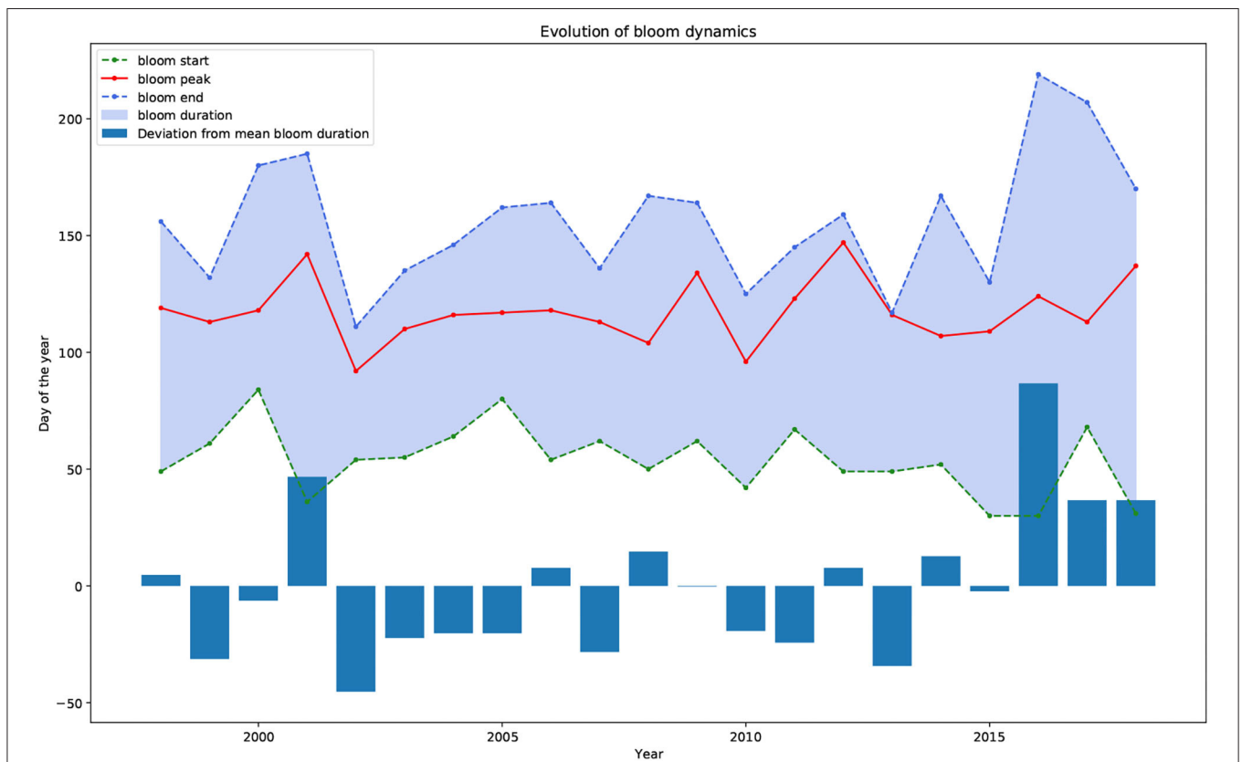
FIGURE 12 | Historical spring bloom cardinal dates (beginning—green, peak—red, end—blue) and bloom duration (shaded blue area). The bar chart shows the yearly deviation (anomaly) from the long-term mean bloom duration.
