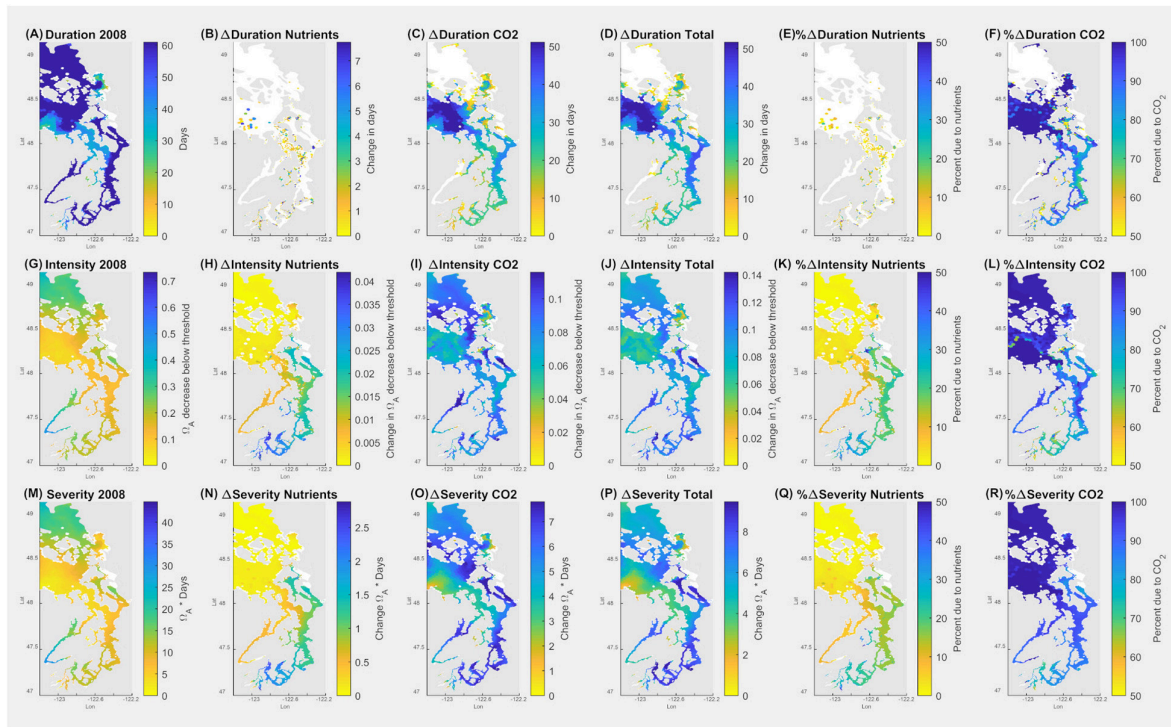
FIGURE 7 | Application of pteropod threshold for growth impairment (7 days at \Omega_{ar} = 1.0 ) over the seasonal scale in the upper 100 m of the Salish Sea during September–October. Model outputs demonstrate current (2008) duration, intensity, and severity of the conditions ( A,G,M ). The second column indicates the changes due to nutrients ( B,H,N ); the third column depicts the changes due to atmospheric \text{CO}_2 ( C,I,O ); the fourth column ( D,J,P ) shows total changes due to both nutrients and atmospheric \text{CO}_2 . The fifth column ( E,K,Q ) depicts % changes in \Omega_{ar} due to nutrients, and the sixth column ( F,L,R ) is % change in \Omega_{ar} due to atmospheric \text{CO}_2 . Values of zero are masked in white.
