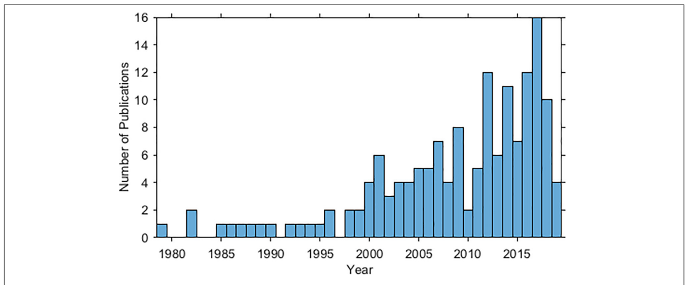
FIGURE 2 | Histogram of the number of publications meeting search criteria—by year (until mid-2019).
