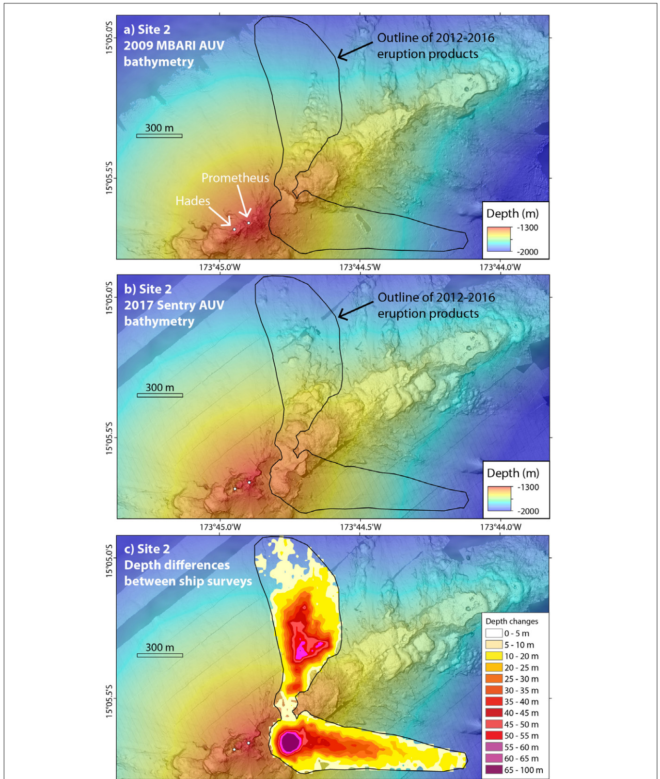
FIGURE 7 | Broad-view maps of eruption site #2, just east of the summit of West Mata (see Figure 2 ) showing (a) pre-eruption MBARI AUV bathymetry from 2009, (b) post-eruption Sentry AUV bathymetry from 2017, and (c) positive depth differences between ship-based surveys in 2012 and 2016 ( Table 2 ). Black outlines enclose the site #2 eruption deposits. White dots show locations of Hades and Prometheus eruptive vents in May 2009.
