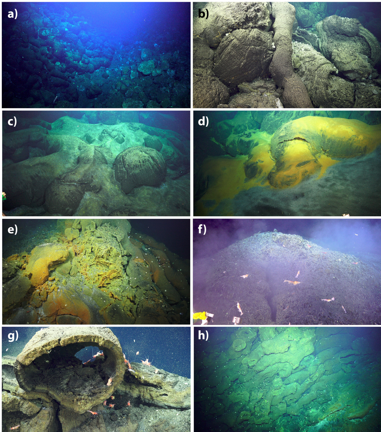
FIGURE 9 | Images of eruption site #2 from ROV SuBastian dives S85, S87, and S103. All show 2012–2016 eruption products. Numbers in parentheses are dive number, time of photo in GMT and horizontal scale. See Figure 8d for photo locations. (a) 2012–2016 flow front at left against the 2010–2011 landslide headwall at right (S85, 01:52:19, 10 m). (b) Close up of pillow lavas on flow front (S85, 01:58:13, 3 m). (c) Tephra partly burying pillows close to eruptive vent (S85, 02:59:14, 5 m). (d) Tephra with white and yellow microbial mats mantling pillows (S85, 03:18:12, 3 m). (e) Near-vent spatter deposits with yellow hydrothermal sediment (S85, 02:50:48, 5 m). (f) Hydrothermal vent shrimp swarm at active diffuse vent with shimmering cloudy water (S87, 03:19:25, 3 m). (g) Hollow drained-out pillow where new lavas are cut by landslide scarp (S103, 02:42:53, 1.5 m). (h) Cross-section of stack of elongate pillow lavas cut by landslide scarp, with downslope direction to the left (S85, 02:45:15, 10 m).
