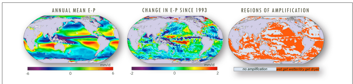
FIGURE 5 | Linking salinity to the global hydrological cycle is one of scientific drivers of satellite SSS. Shown here are mean patterns of the ocean water cycle and its amplification in the last two decades based on the ECCO ocean state estimate. Left: average rates at which freshwater enters (blue) or leaves (red) the ocean via the processes of precipitation (P) and evaporation (E); Middle: trends in E-P; blue (negative) means that the ocean received more freshwater since 1993. Right: Amplification of the ocean water cycle, computed as a slope of the linear regression between the anomalies and trends in E-P. Pattern amplification is shown as orange, otherwise is shaded gray. In many ocean regions, pattern amplification follows the wet gets wetter/dry gets drier paradigm, as more freshwater is brought to wet regions (e.g., blue colors match blue in the tropics), or more freshwater is removed from dry regions (e.g., red colors match red in the United States west coast. If averaged over the globe, the ocean water cycle has amplified by 5% since 1993. See Vinogradova and Ponte (2017) for details.
