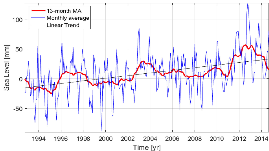
FIGURE 6 | Regional sea level variations over 1993–2015. Monthly averaged values are shown in blue and 13-month averaged values are shown in red.
