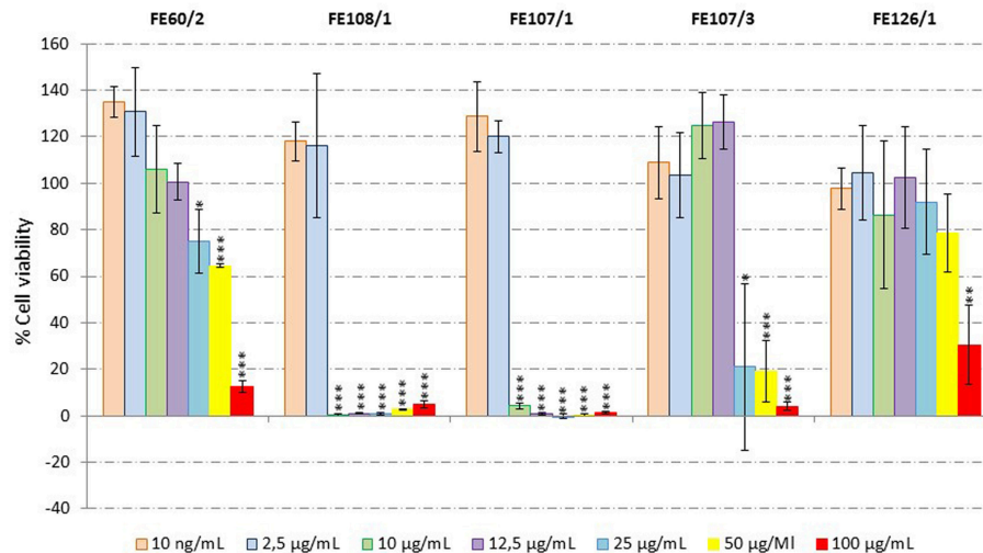
FIGURE 3 | Anticancer Assay. Percentage viability of human melanoma cells (A2058) after incubation for 72 h with microalgal extracts ( Skeletonema marinoi FE60/2, Alexandrium andersoni FE108/1, Alexandrium tamutum FE107/1 and FE107/3, and Alexandrium minutum FE126/1) at 100, 50, 25, 12.5, 10, and 2.5 µg/mL and 10 ng/mL ( n = 9 , data represent means for three biological and nine technical triplicates; * for p < 0.05 , ** for p < 0.01 and *** for p < 0.001 , Student's t -test) compared to control.
