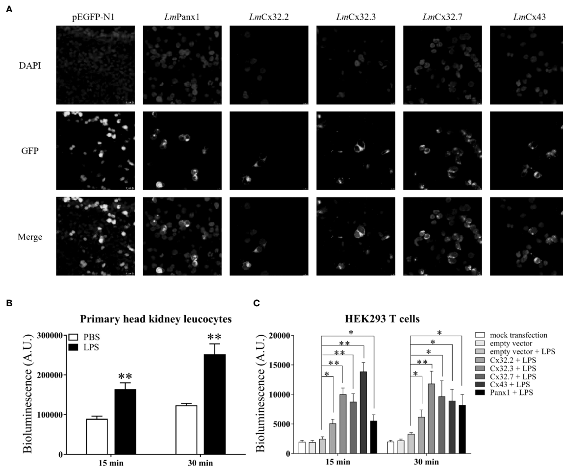
FIGURE 8 | Subcellular localization of LmPanx1 , LmCx32 , and LmCx43 in HEK293 T cells (A) and LPS-induced extracellular ATP release in primary head kidney leukocytes (B) or HEK293 T cells (C) . (A) HEK293 T cells were transfected with pEGFP-N1- LmPanx1 , pEGFP-N1- LmCx32.2 , pEGFP-N1- LmCx32.3 , pEGFP-N1- LmCx32.7 , or pEGFP-N1- LmCx43 plasmids. At 24 h posttransfection, the cells were stained with DAPI and observed under a confocal microscope. (B, C) The primary head kidney leukocytes were stimulated with LPS (100 \mu\text{g}/\text{mL} ) or PBS (control). HEK293 T cells were transfected with pcDNA3.1- LmPanx1 , pcDNA3.1- LmCx32.2 , pcDNA3.1- LmCx32.3 , pcDNA3.1- LmCx32.7 , or pcDNA3.1- LmCx43 . After 24 h, the cells were stimulated with LPS (100 \mu\text{g}/\text{mL} ). The supernatant was collected at 15 and 30 min after stimulation and the ATP levels were subsequently measured. The mock transfected and empty plasmid transfected cells served as controls. Data are shown as mean \pm SEM (N = 4). * p < 0.05 , ** p < 0.01 are considered significant difference.
