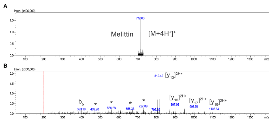
FIGURE 5 | Representative mass spectrometry profile for the qualitative assessment of the presence of melittin in the serum of participant 115, considered positive (+++): (A) Melittin [M+4H] 4+ MS profile and (B) MS 2 interpreted profile, annotated for the larger b and y ions, as well as internal fragments (*).
