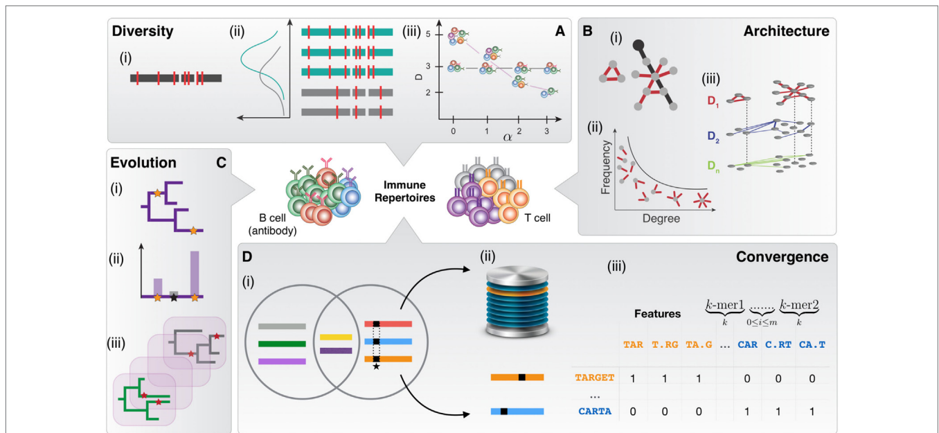
FIGURE 1 | The immune repertoire space is defined by diversity, architecture, evolution, and convergence. (A) Diversity measurements are based on (i) the accurate annotation of V (D) J segments using deterministic and probabilistic approaches with population-level or individualized germline gene reference databases. (ii) Probabilistic and hidden Markov models allow inference of recombination statistics. (iii) Measurement of clonotype diversity using diversity profiles. (B) Analysis of repertoire architecture relies predominantly on (i) clonal networks that are constructed by connecting nucleotide or amino acid sequence nodes by similarity edges. The sequence similarity between clones is defined via a string distance [e.g., Levenshtein distance (LD)], resulting in undirected Boolean networks for a given threshold (nucleotides/amino acids). An example of the global characterization of the network is the diameter, shown by black edges. An example of the local parameters of the network is the degree ( n = 1 ) related to the individual clonal node in black. (ii) Degree distribution is a global characteristic of immune repertoire networks, which can be used for analyzing clonal expansion. (iii) Several similarity layers decompose the immune repertoire along its similarity layers. Layer D1 captures clonal nodes similar by edit distance 1 (1 nt/a.a. different), D2 of distance 2 and so forth. (C) Assessing evolution of antibody lineages. (i) Reconstruction of phylogenetic trees. Stars indicate somatic hypermutation. (ii) Probabilistic methods for the inference of mutation statistics in antibody lineage evolution. (iii) Simulation of antibody repertoire evolution for benchmarking antibody-tailored phylogenetic inference algorithms. (D) Naive and antigen-driven cross-individual sequence similarity and convergence in immune repertoires. (i) The Venn diagram shows sequences shared in the two repertoires (circles). Signature-like sequence features are highlighted by black squares. (ii) Database of convergent or antigen-specific immune receptor sequences. (iii) K-mer sequence decomposition and classification of immune receptor sequences.
