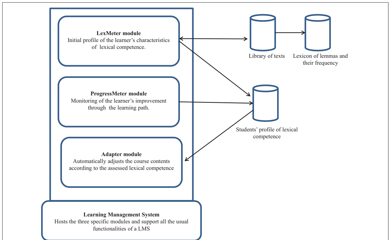
FIGURE 1 | The overall structure of the Am-learning system.
