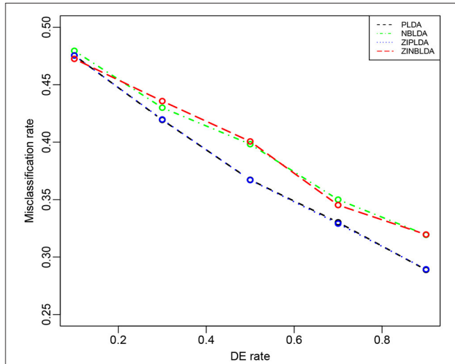
FIGURE 6 | The misclassification rates of the four methods with different probabilities of differential expression genes (Study 5). Here, \sigma = 0.2 , p = 100 , n = 8 , \phi = 0.5 , and p_0 = 0 .
